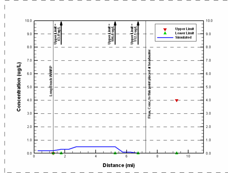
Figure 31. Simulated vs. observed Total Lead of Coyote Creek in September 2003 (zero for non-detects)
