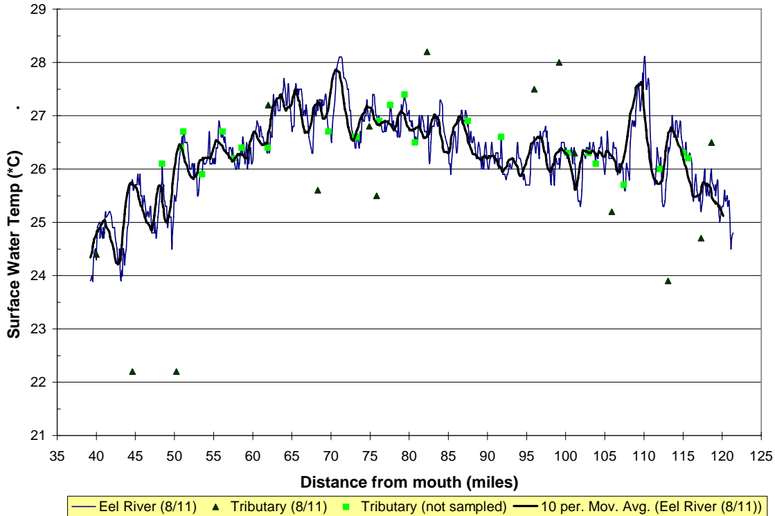
Figure 7 - Longitudinal profile with both sampled and detected (not sampled) tributaries along Middle Main Eel River. The plot also shows a moving average trend line derived from the sampled data.
