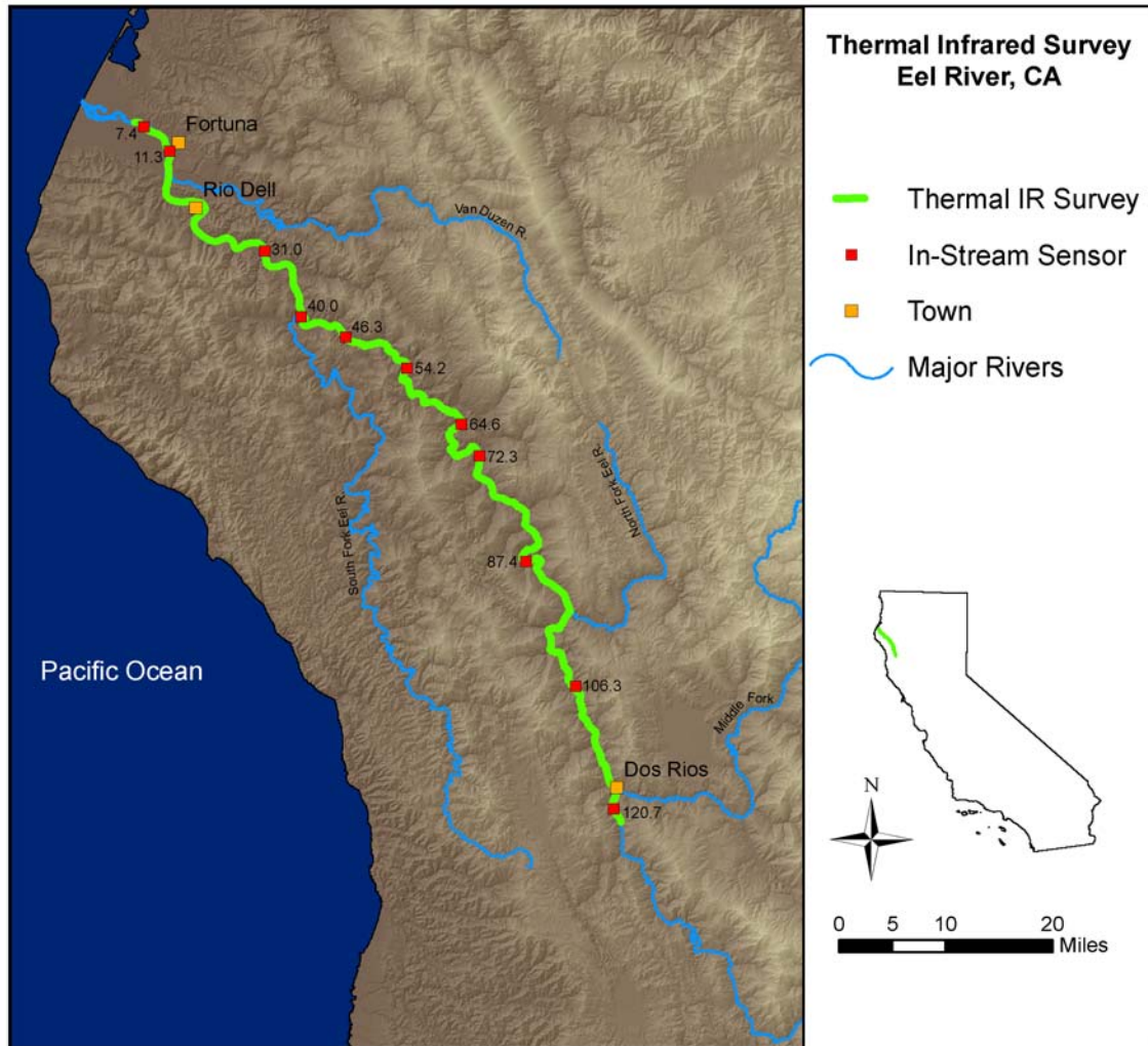
Figure 1 – Map showing the extent of the airborne thermal infrared survey on the Eel River on August 11-12, 2005. The map also shows the location of in-stream temperature monitors labeled by river mile.
