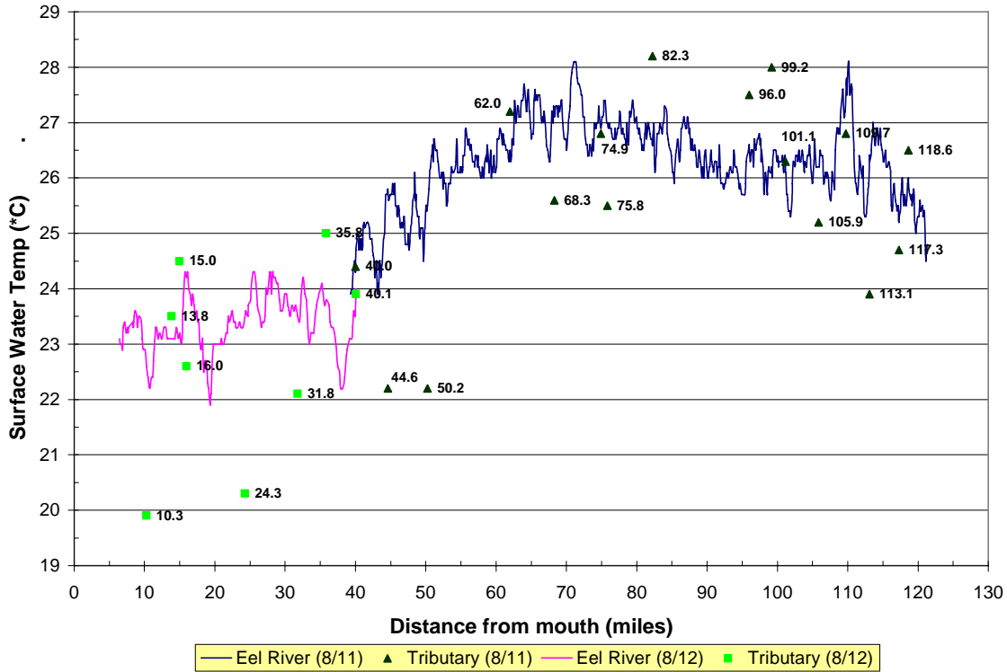
Figure 6 - Median sampled temperatures plotted versus river mile for the Eel River. Tributaries and other sampled inflows (i.e. springs/seeps, irrigation returns) are labeled on the profile by river mile
