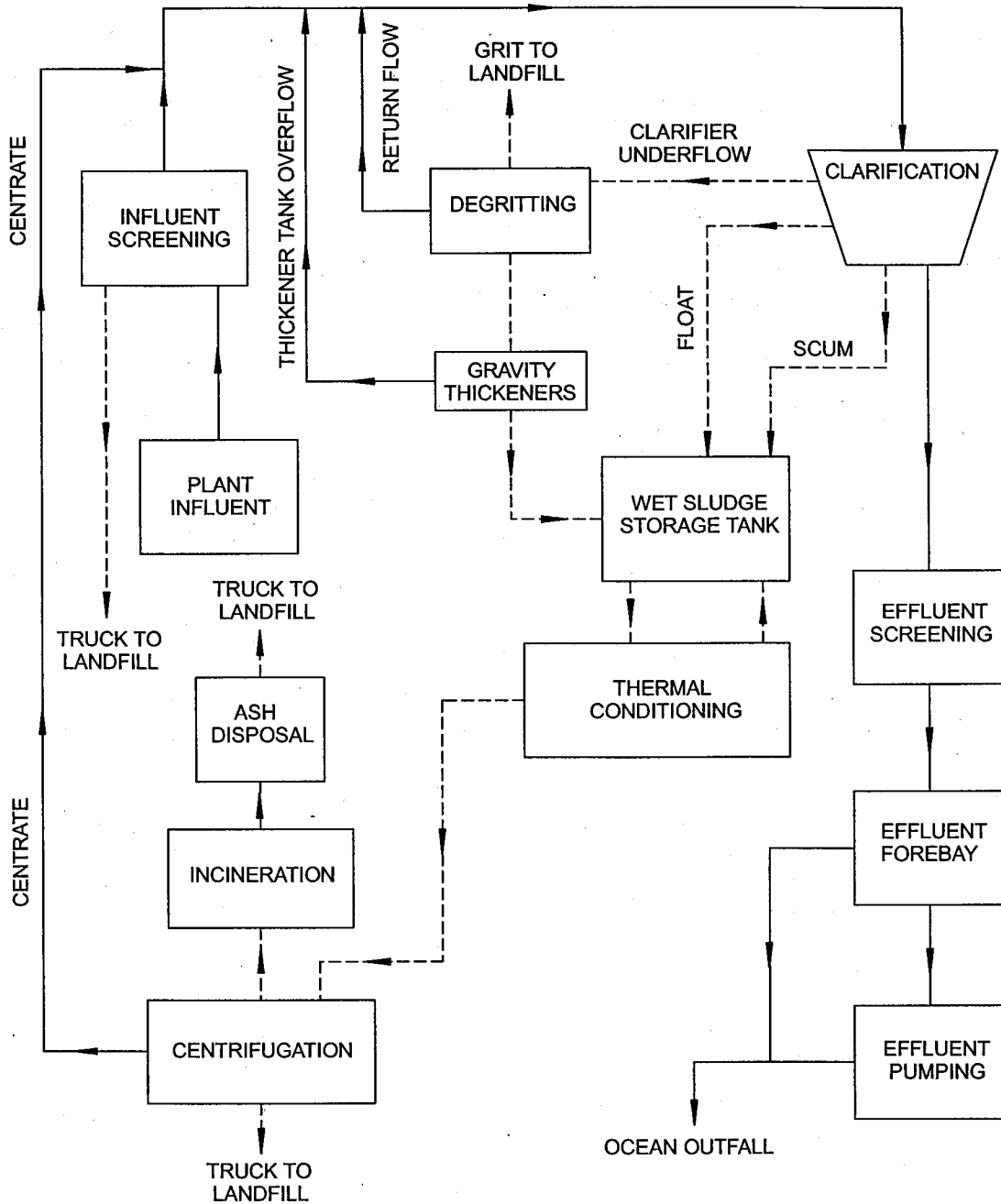
FIGURE 4A LIQUID & SOLID FLOW SCHEMATIC
