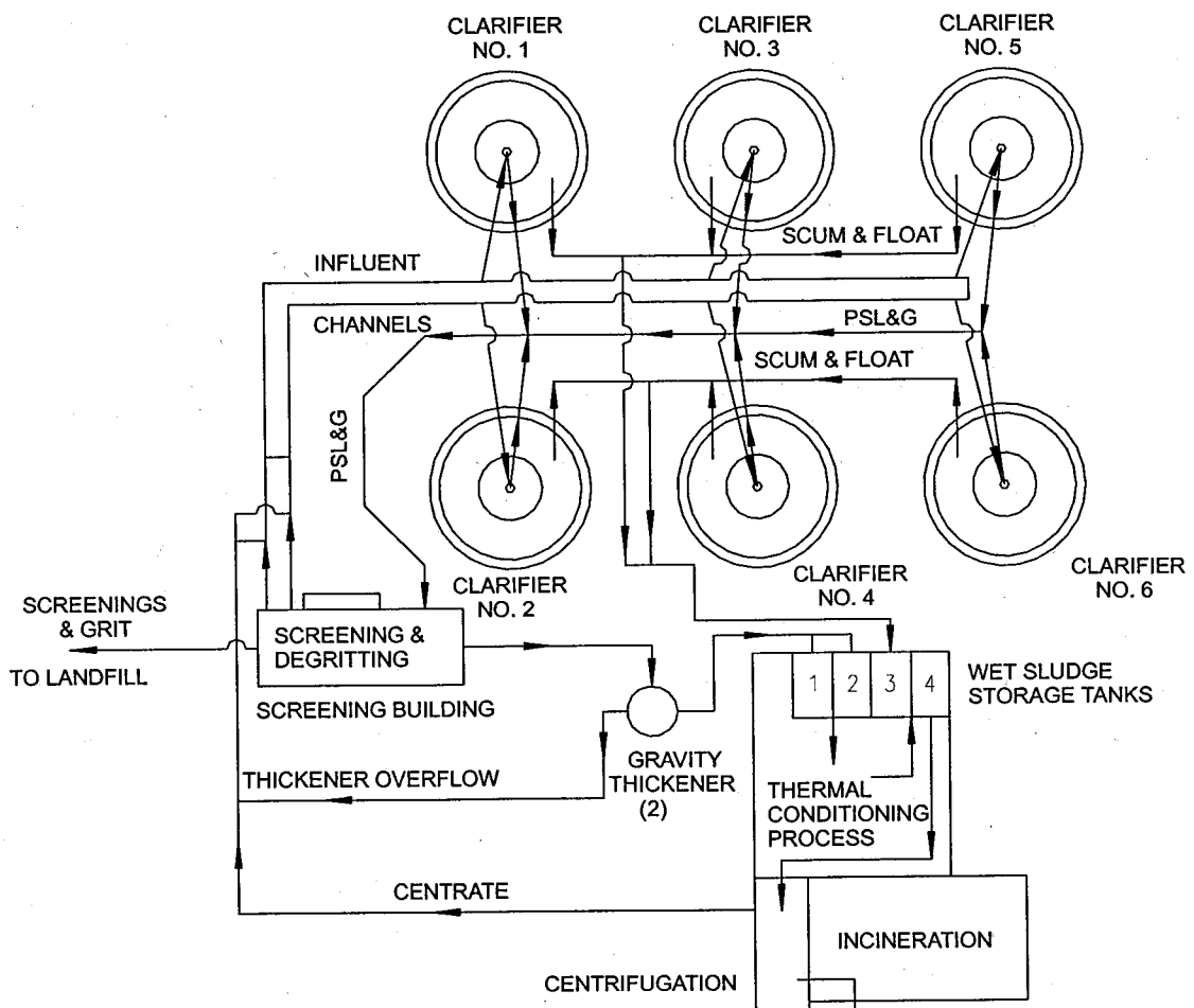
FIGURE 3A SOLIDS FLOW DIAGRAM FOR REMOVAL BY DISSOLVED AIR FLOTATION
