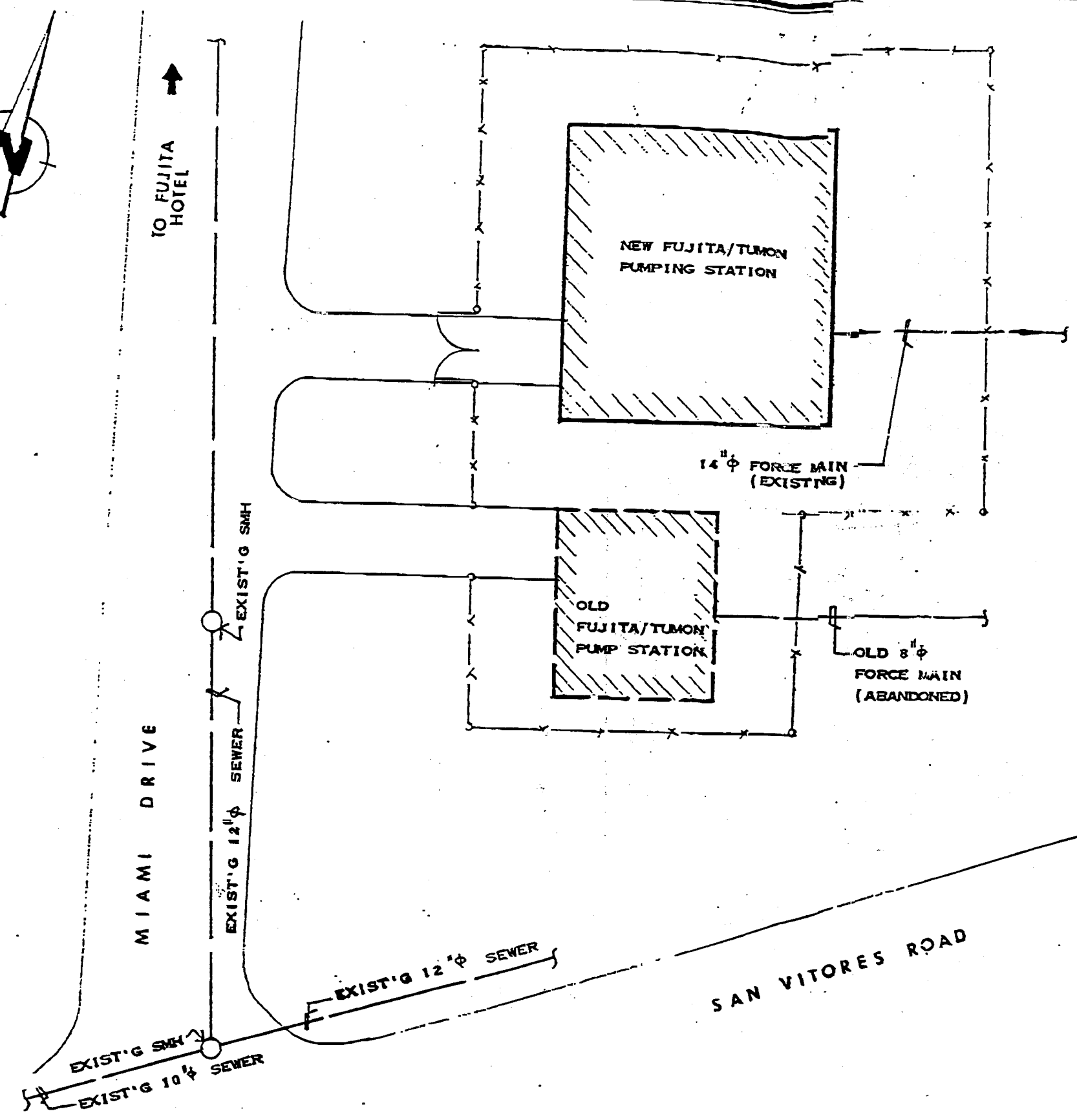
FIGURE 3 SITE PLAN- FUJITA PUMP STATION
