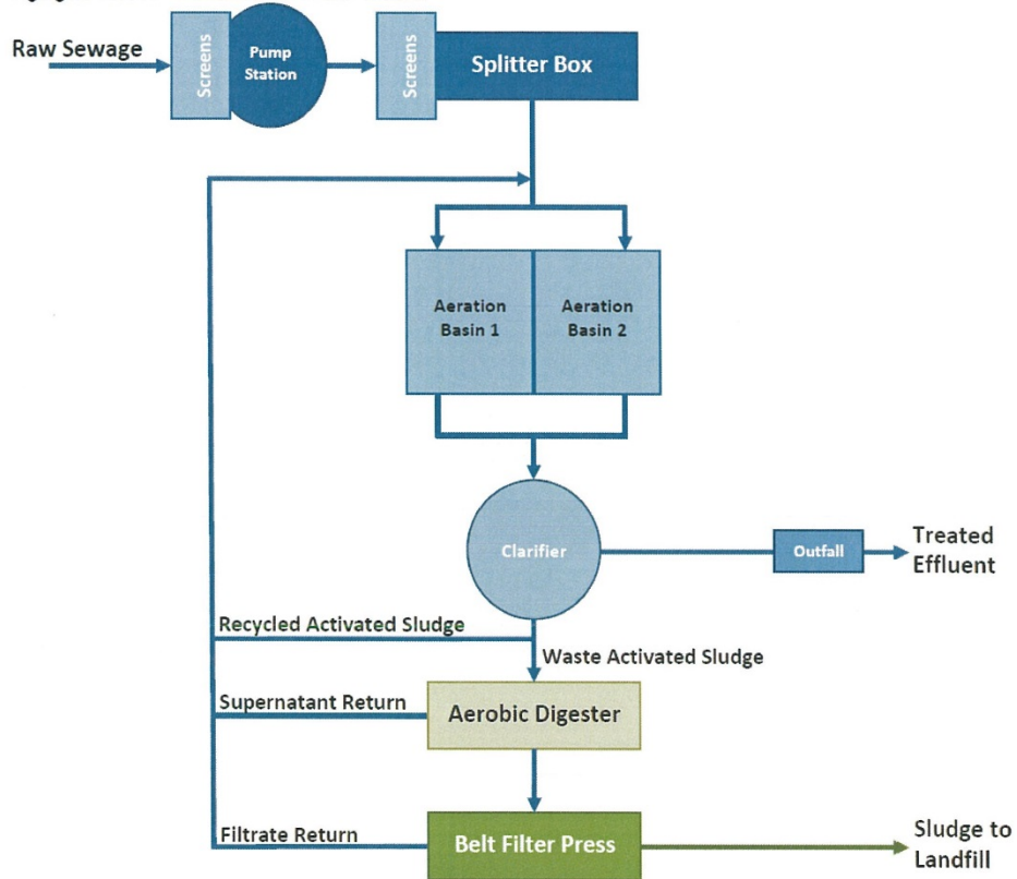
FIGURE 4 Agingan WWTP Treatment Process Outline
