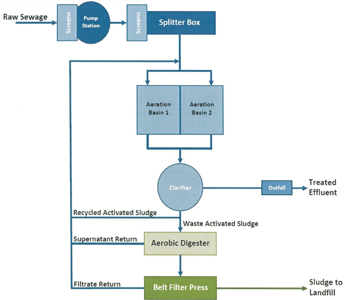
FIGURE 4 WWTP Treatment Process Outline
