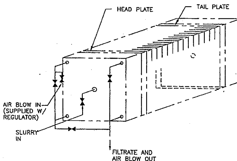
Fig. 4-14. Air Blow Down Manifold Diagram
