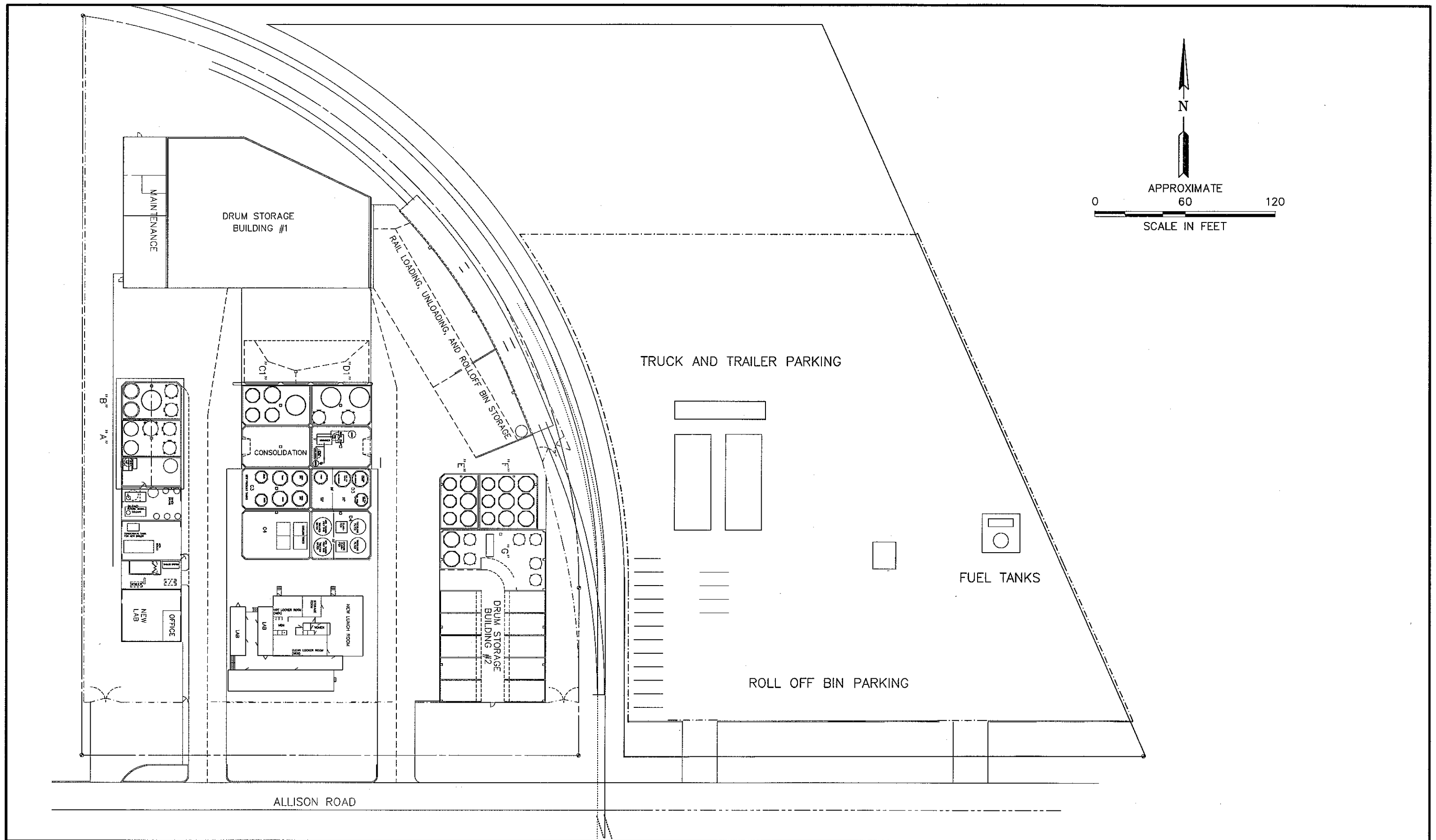
Facility Layout/Site Plan Romic - Southwest Chandler, Arizona Figure B-2
