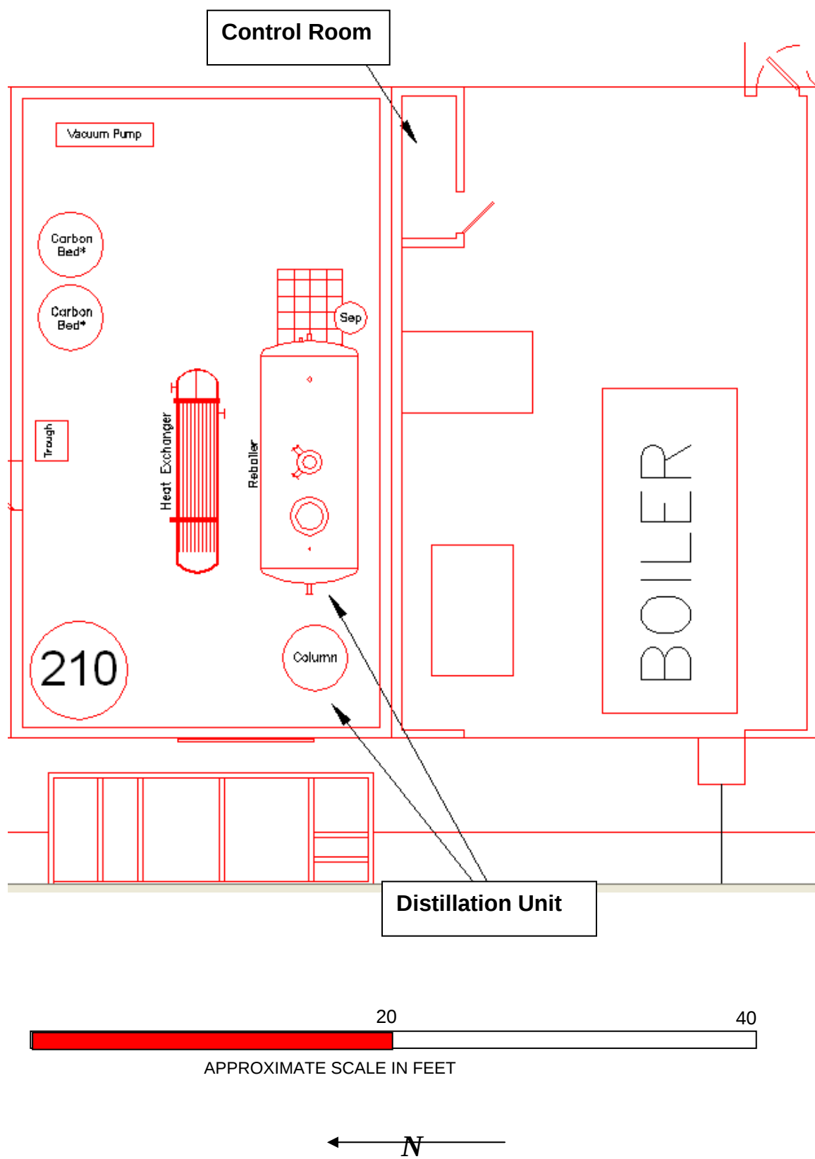
Figure B-9 Distillation Unit
