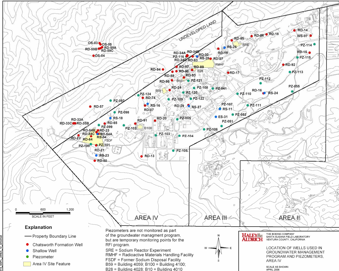
Figure 6-2. Well Locations
