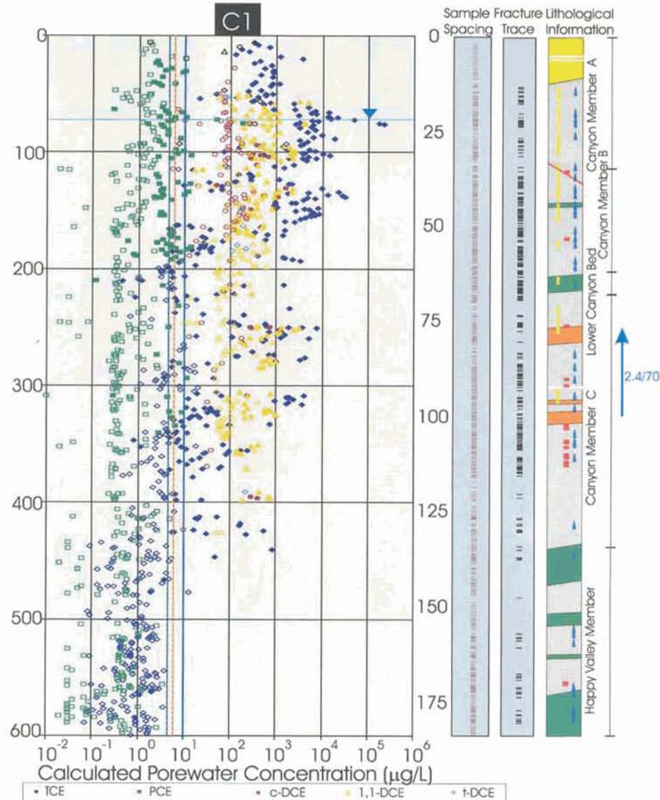
Figure 44. C1 (Instrument Equipment Lab) Profile of TCE Porewater Concentrations Solid lines represent analyte maximum contaminant levels for drinking water for the state of California. Open symbols represent values that are estimates (fall between the method detection limit and the method reporting limit). Solid symbols represent quantitative values. Non-detects are not plotted. All concentrations are below TCE solubility (~1.4x10 6 µg/L porewater).
