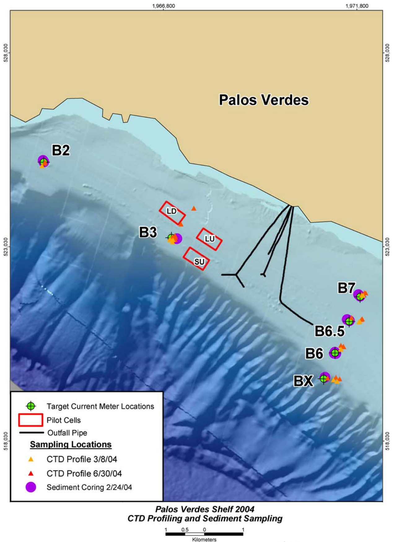
FIGURE 2-5 Mooring Locations for Oceanographic Measurement Program Palos Verdes Shelf Study Area Remedial Investigation Report
