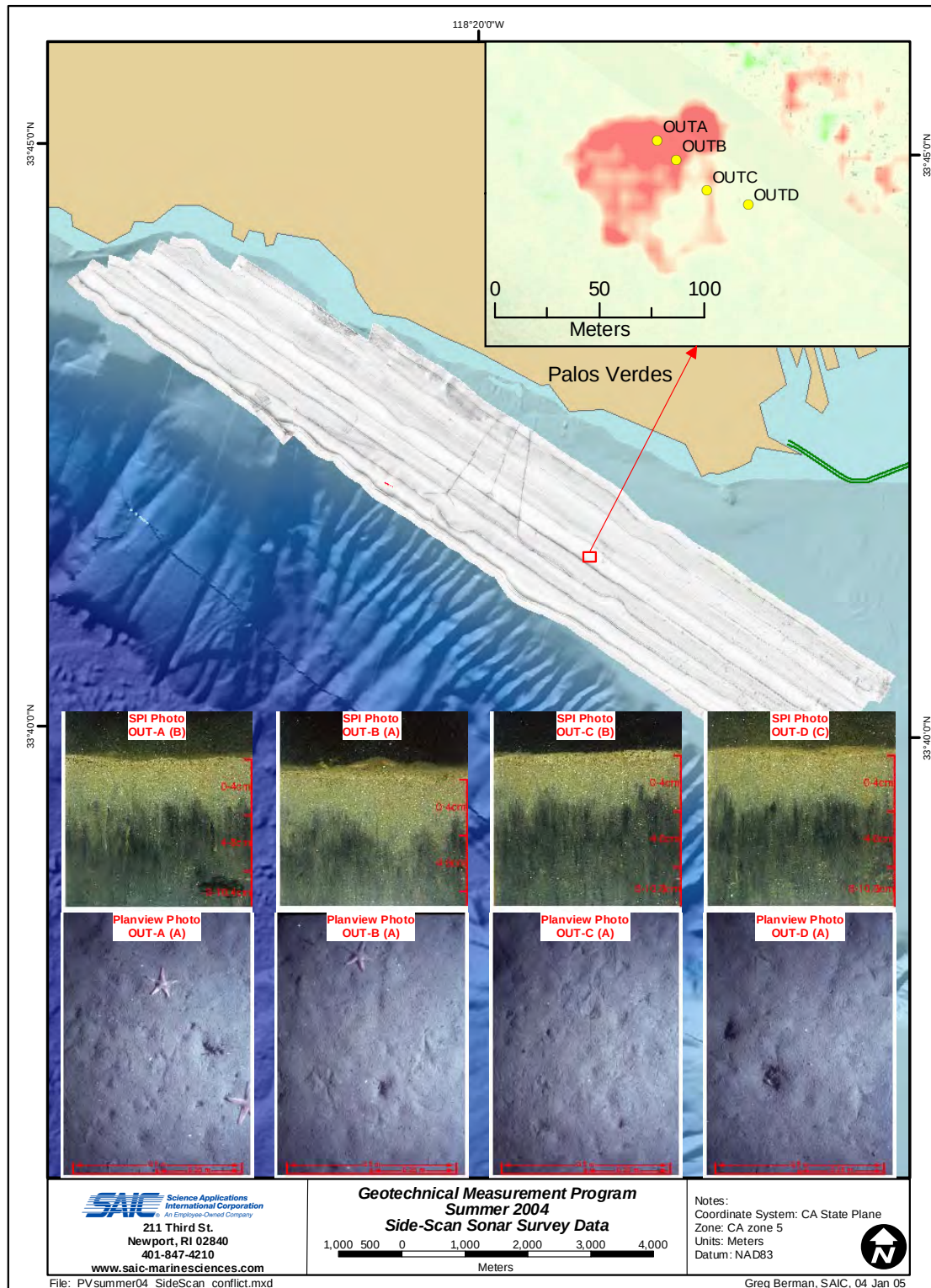
Figure 3.1-6. Sediment-profile and plan-view images relative to the side-scan sonar mosaic. High intensity backscatter returns suggest a hard bottom environment, however both sediment-profile and plan-view images display a soft-bottom habitat.
