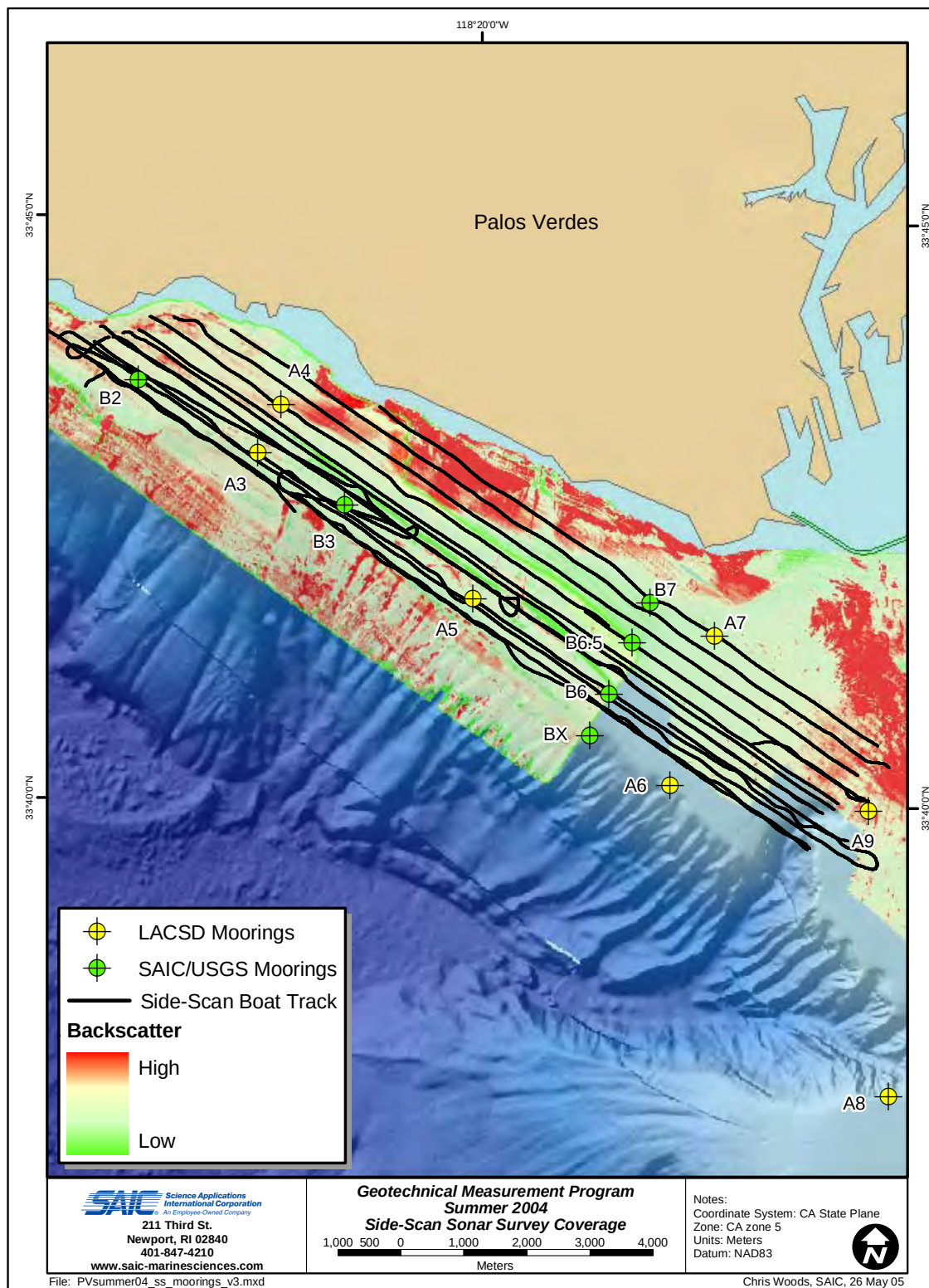
Figure 2.1-1. Overview of side-scan sonar survey lanes that were occupied during the 2004 Geotechnical Measurement Program.
