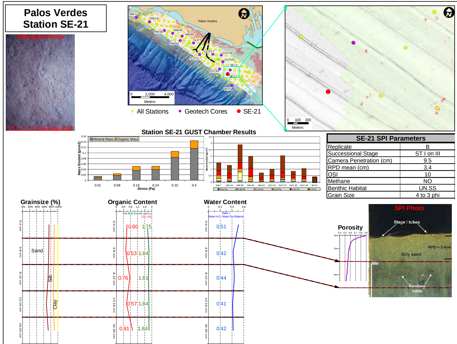
Figure 3.3-26. Composite overview of the analysis results for Station SE-21. The relative location of this sampling station is indicated on the overview graphic at the top of this figure. The graphic in the upper right-hand corner shows the side-scan sonar and multibeam backscatter imagery in the immediate vicinity of this station.
