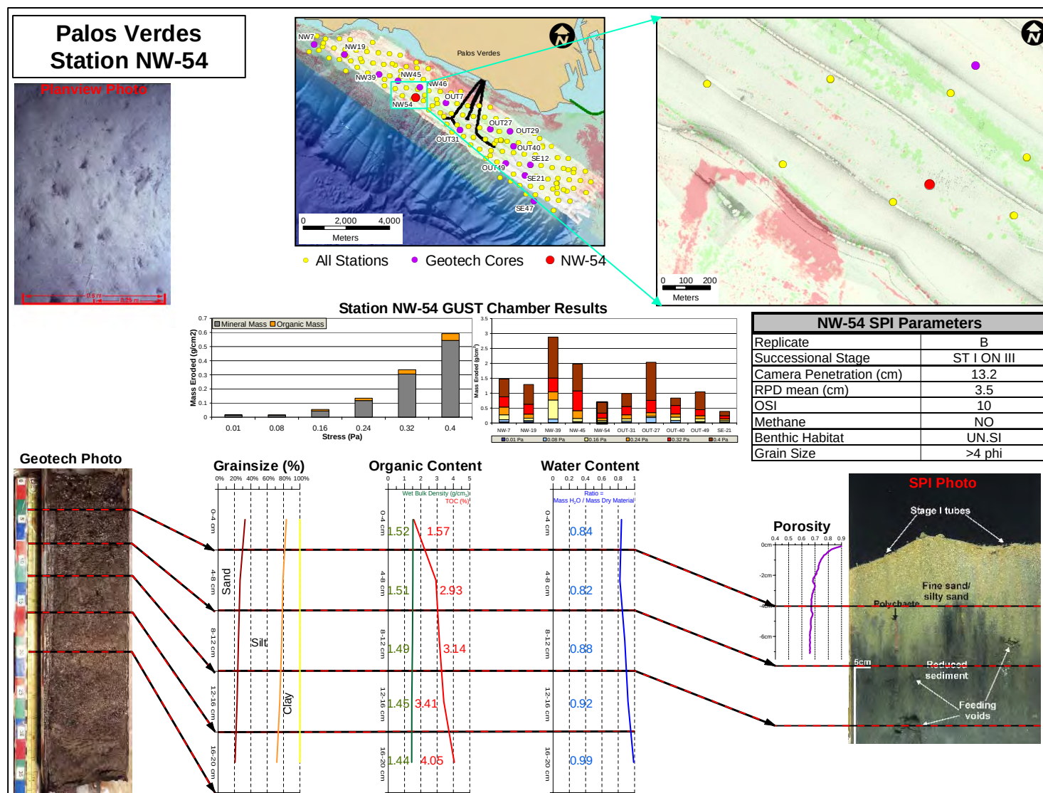
Figure 3.3-18. Composite overview of the analysis results for Station NW-54. The relative location of this sampling station is indicated on the overview graphic at the top of this figure. The graphic in the upper right-hand corner shows the side-scan sonar and multibeam backscatter imagery in the immediate vicinity of this station.
