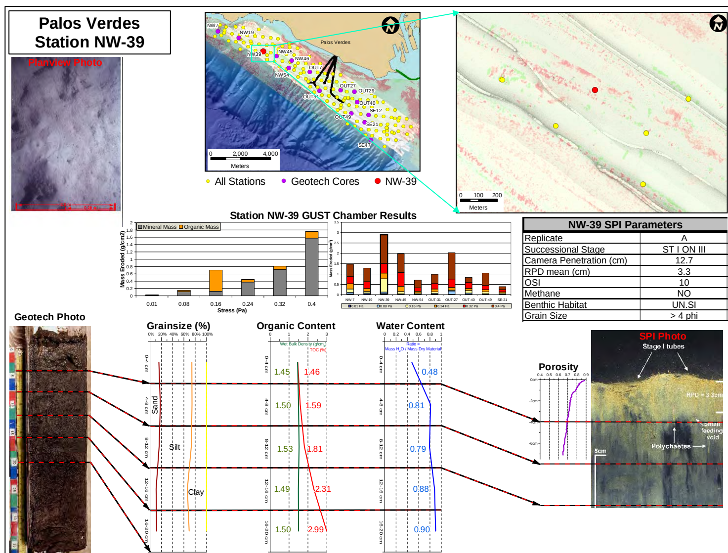
Figure 3.3-15. Composite overview of the analysis results for Station NW-39. The relative location of this sampling station is indicated on the overview graphic at the top of this figure. The graphic in the upper right-hand corner shows the side-scan sonar and multibeam backscatter imagery in the immediate vicinity of this station
