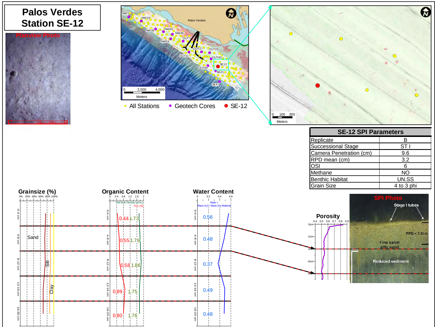
Figure 3.3-25. Composite overview of the analysis results for Station SE-12. The relative location of this sampling station is indicated on the overview graphic at the top of this figure. The graphic in the upper right-hand corner shows the side-scan sonar and multibeam backscatter imagery in the immediate vicinity of this location.
