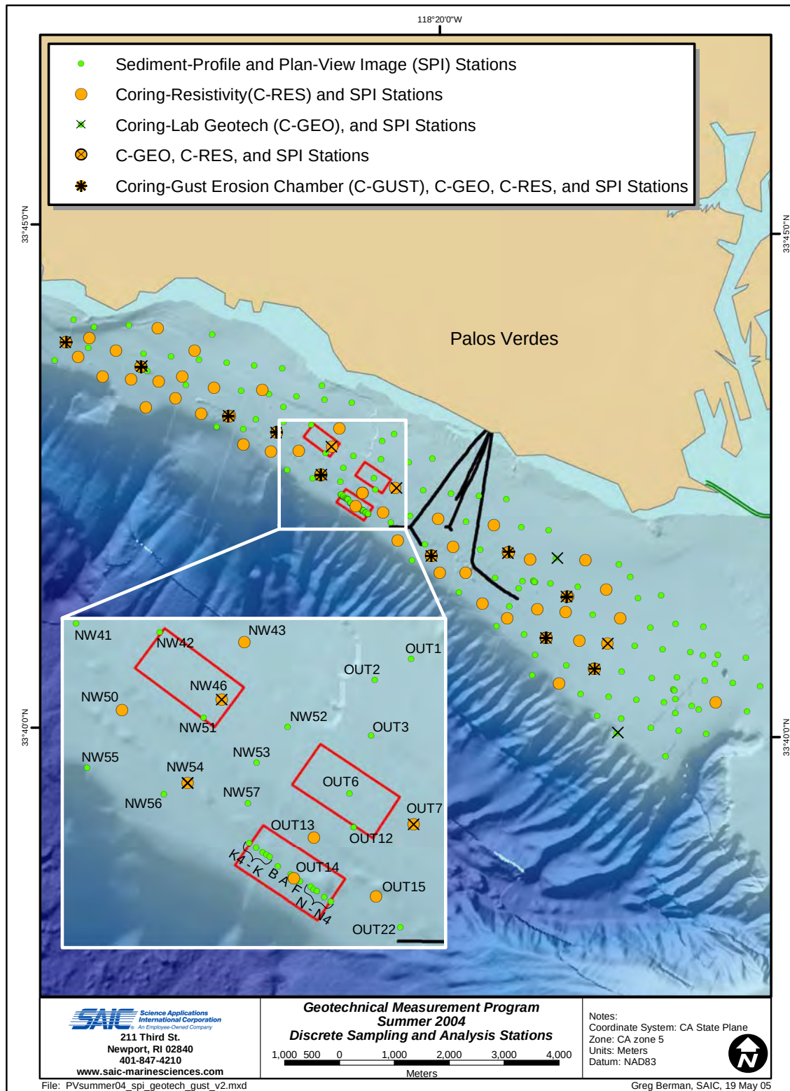
Figure 2.2-1. Overview of imaging and geotechnical discrete sampling stations that were occupied during the 2004 Geotechnical Measurement Program.
