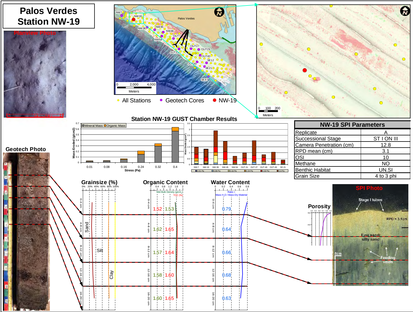
Figure 3.3-14. Composite overview of the analysis results for Station NW-19. The relative location of this sampling station is indicated on the overview graphic at the top of this figure. The graphic in the upper right-hand corner shows the side-scan sonar and multibeam backscatter imagery in the immediate vicinity of this station.
