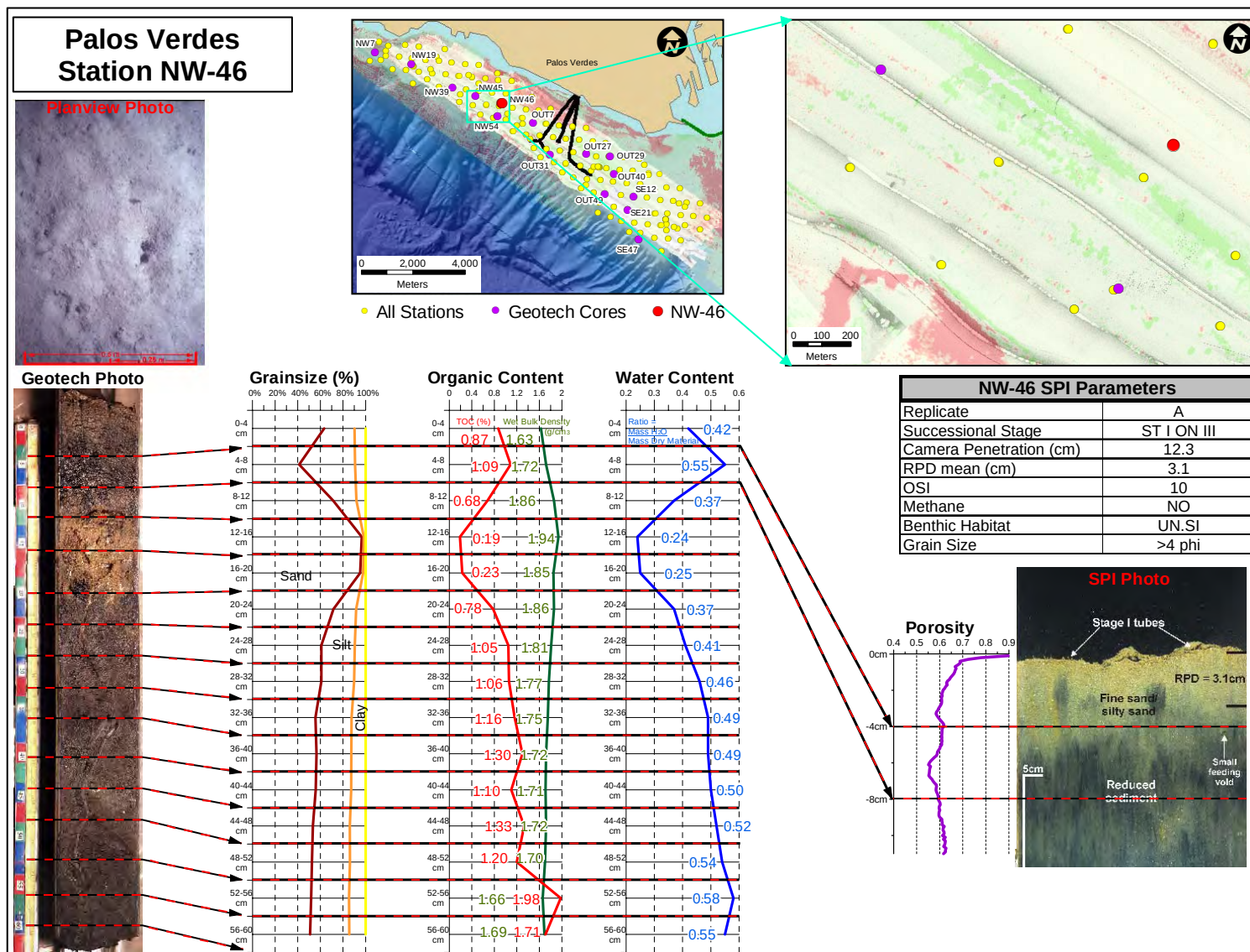
Figure 3.3-17. Composite overview of the analysis results for Station NW-46. Because this station was within one of the pilot cap cells, (LD), it was sub-sampled for its entire length. The relative location of this sampling station is indicated on the overview graphic at the top of this figure. The graphic in the upper right-hand corner shows the side-scan sonar and multibeam backscatter imagery in the immediate vicinity of this station.
