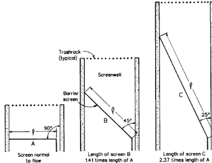
Figure 4.24 Cross-channel Distance of Louver Systems [Ref. 6.110]
