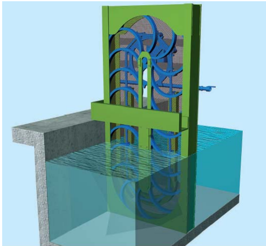
Figure 4.7 Geiger MultiDisc® Screen [Ref. 6.96]
