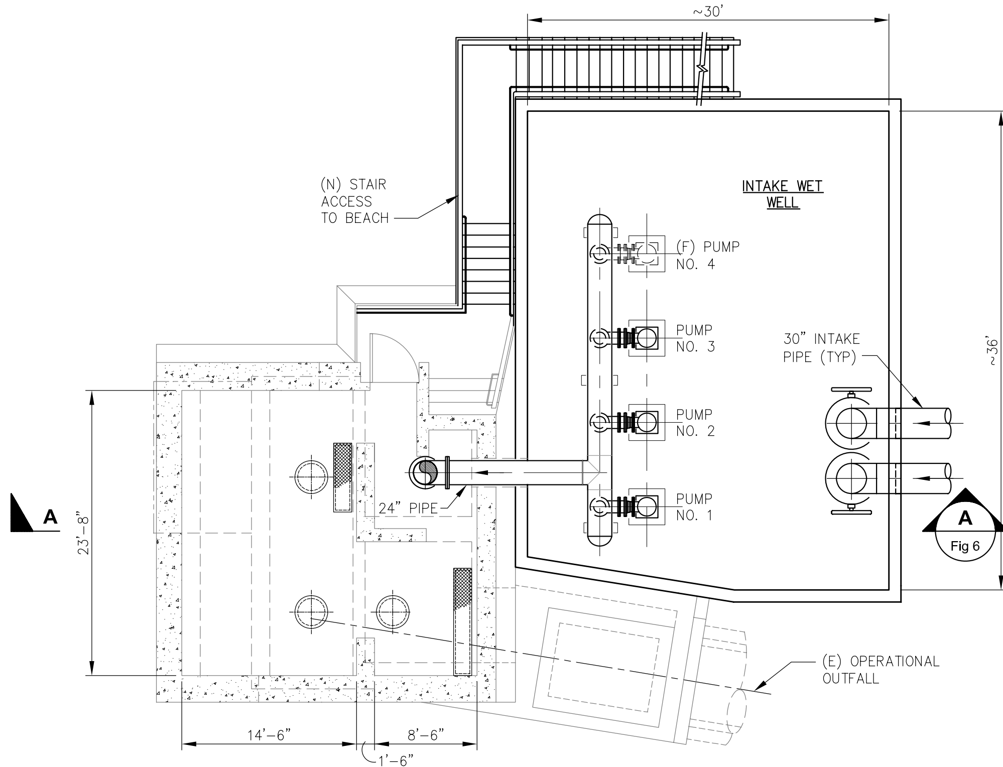
PLAN AT EL. 22.00 SCALE: 1/8" = 1'-0"
