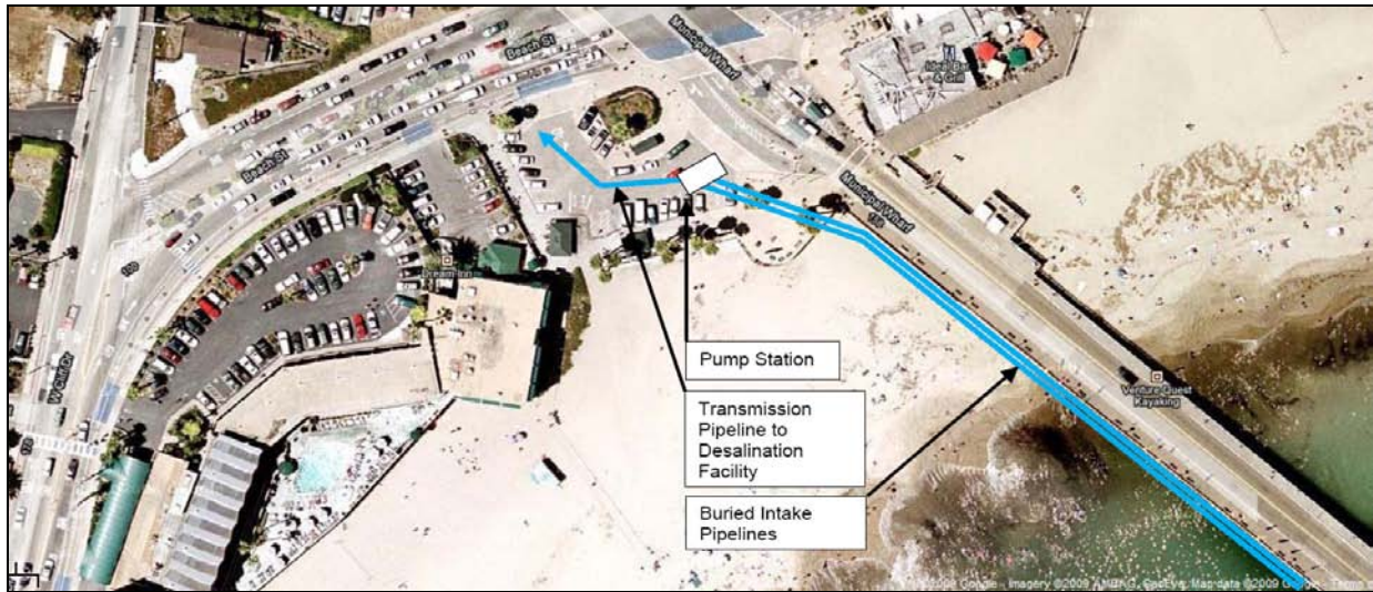
Figure 11-5: Conceptual Municipal Wharf-Located Intake Pipelines and Pump Station Aerial View
