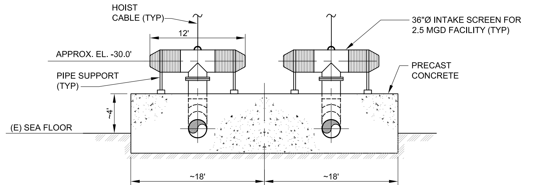
SECTION - A NO SCALE
