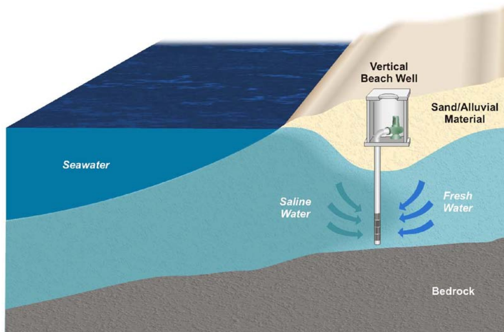
Figure 3-1: Graphic of a Vertical Beach Well
