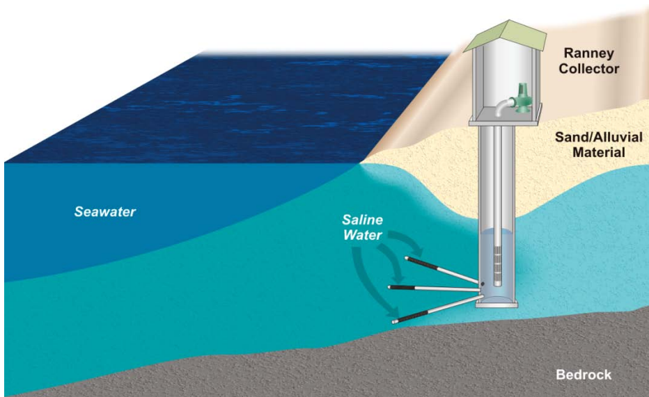
Figure 3-4: Graphic of a Horizontal Collector Well
