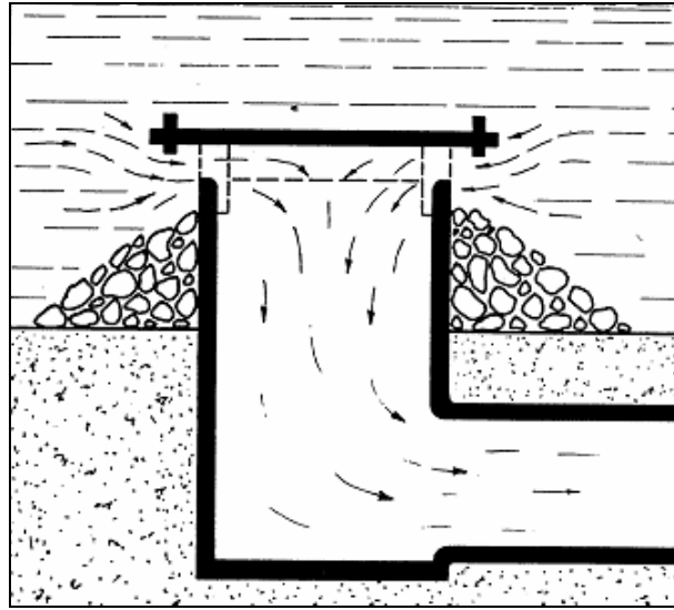
Figure 8-1: Velocity Cap at the Terminus of an intake Pipe
