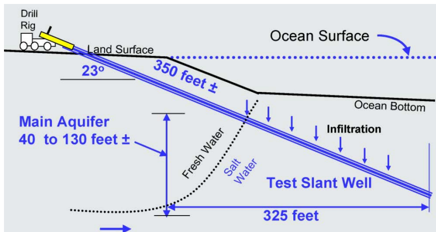
Figure 3-2: Graphic of a Slant Well Extending Out into a Marine Alluvial Channel (MWDOC, 2007)
