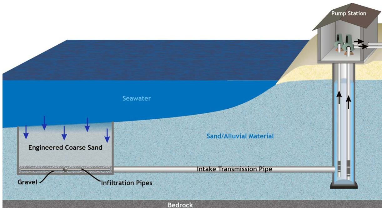
Figure 3-6: Graphic of an Engineered Infiltration Gallery
