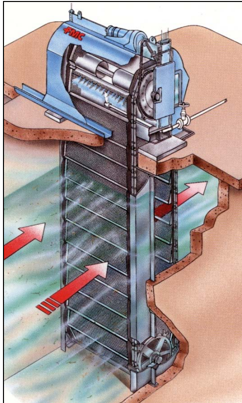
Figure 8-3: Fine-mesh Traveling Water Screen
