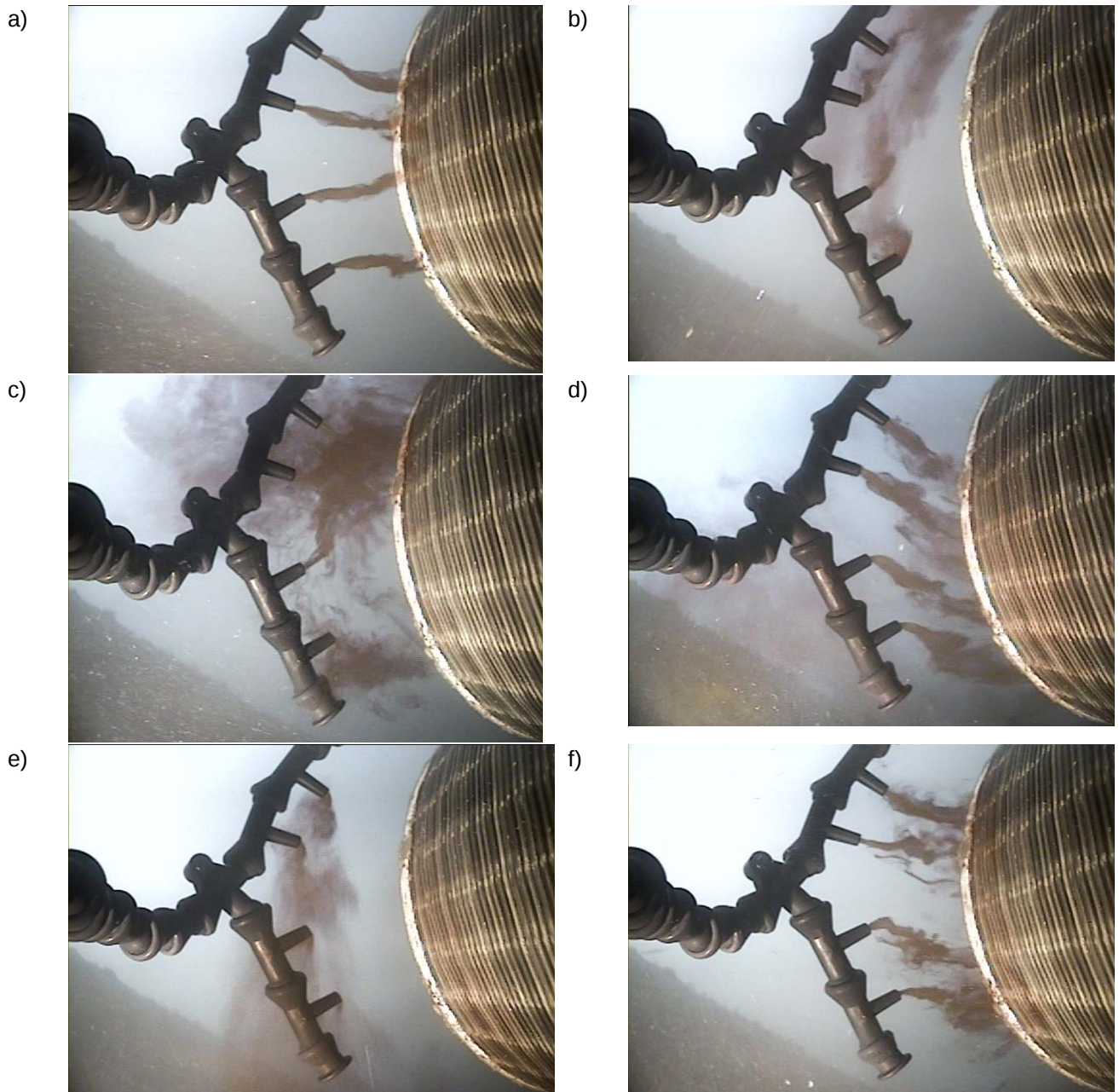
Figure 9-7: Dye Testing Showing Currents Interacting with the Intake Screen (Tenera, 2010)
