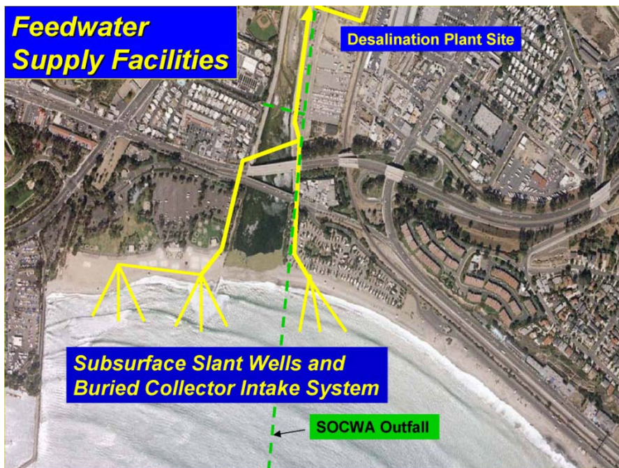
Figure 3-3: Concept for MWDOC's Sub-Seafloor Slant Well Intake System (MWDOC, 2007)
