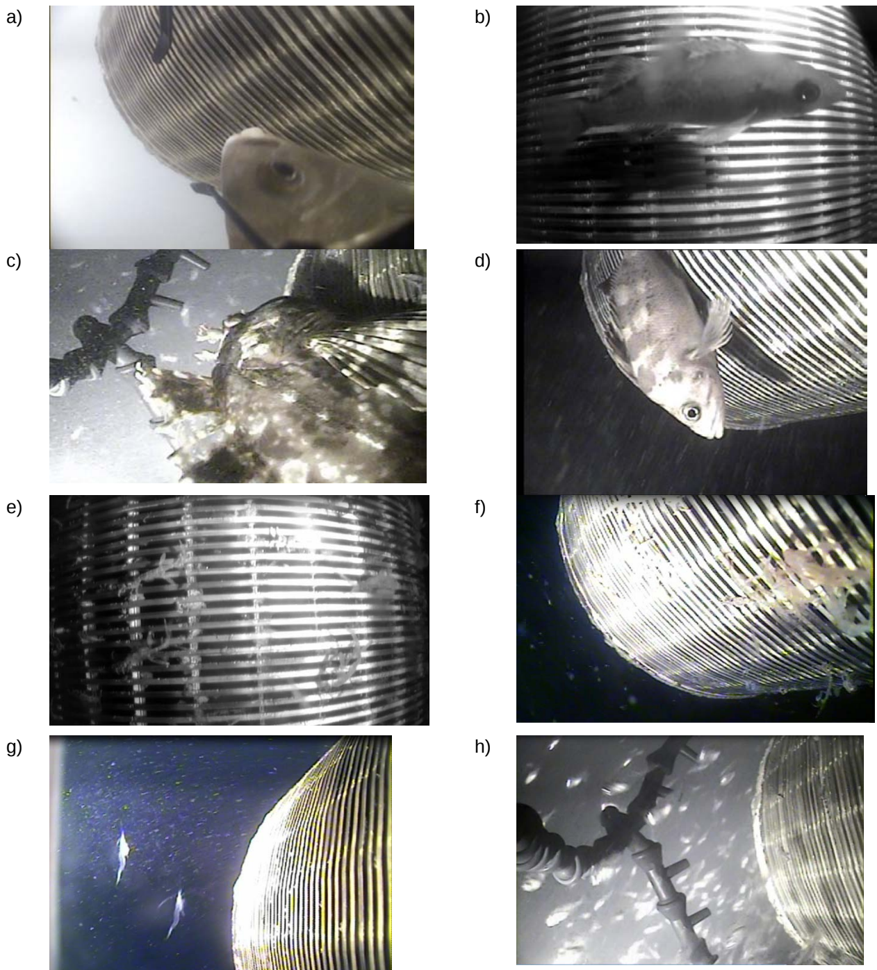
Figure 9-6: Photographs Taken during Wedgewire Screen Pilot Study with Pump Operating (Tenera, 2010)
