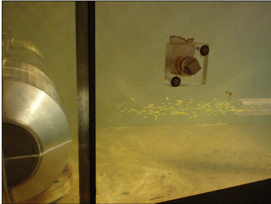
Figure 2-1: Laboratory Evaluation of a Narrow-Slot Cylindrical Wedgewire Screen (EPRI, 2003)
