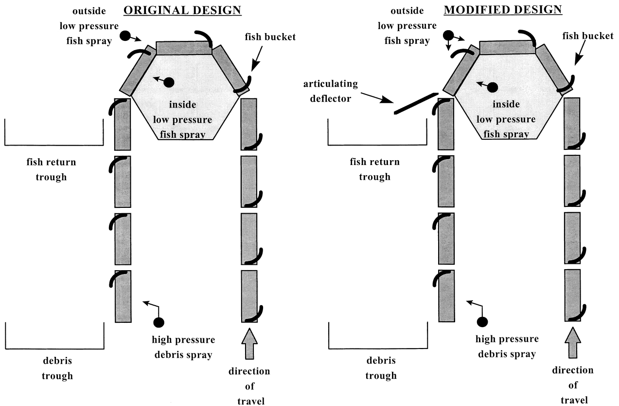
Fig. 1. Schematic cross-section of the traveling screen systems installed at Somerset Station, showing the original (left) and modified (right) designs.
