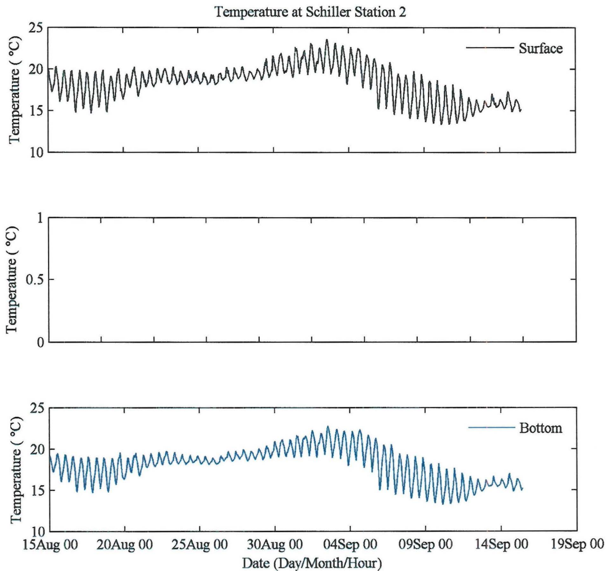
Figure 3. Plotted water temperature data recorded at locations A (surface) and C (bottom) at Station 2 for the Schiller Station thermal monitoring for the period 15 August through 15 September 2010.
