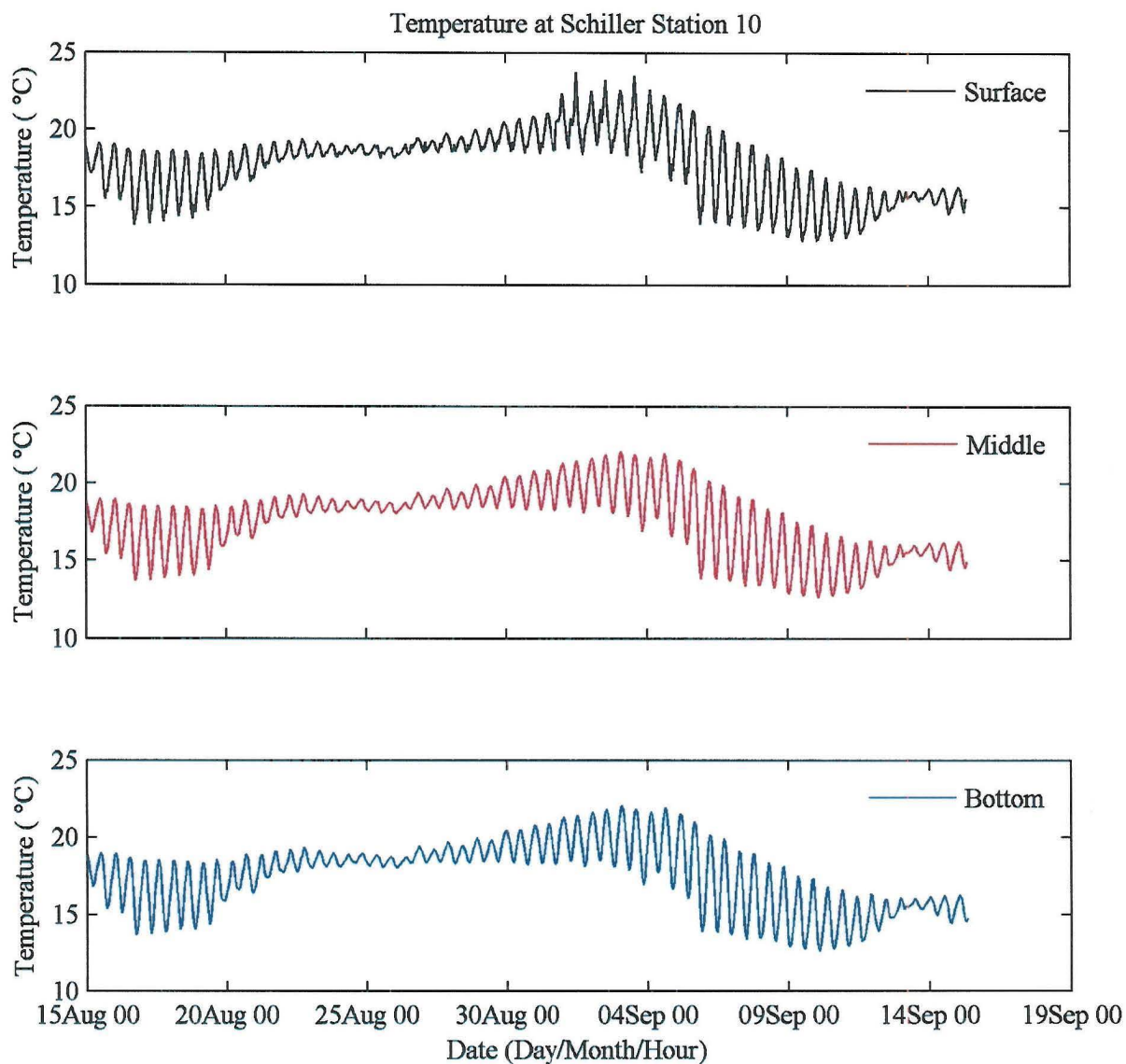
Figure 11. Plotted water temperature data recorded at locations A (surface), B (mid-depth) and C (bottom) at Station 10 for the Schiller Station thermal monitoring for the period 15 August through 15 September 2010.
