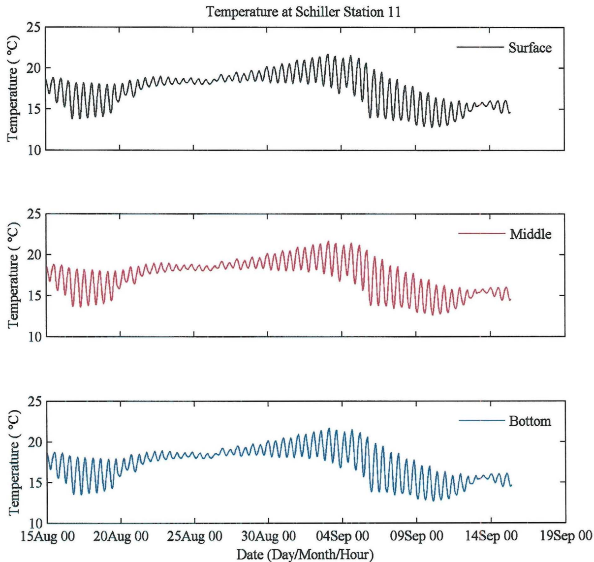
Figure 12. Plotted water temperature data recorded at locations A (surface), B (mid-depth) and C (bottom) at Station 11 for the Schiller Station thermal monitoring for the period 15 August through 15 September 2010.
