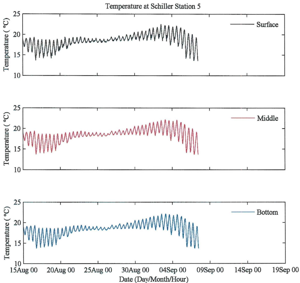
Figure 6. Plotted water temperature data recorded at locations A (surface), B (mid-depth) and C (bottom) at Station 5 for the Schiller Station thermal monitoring for the period 15 August through 15 September 2010.
