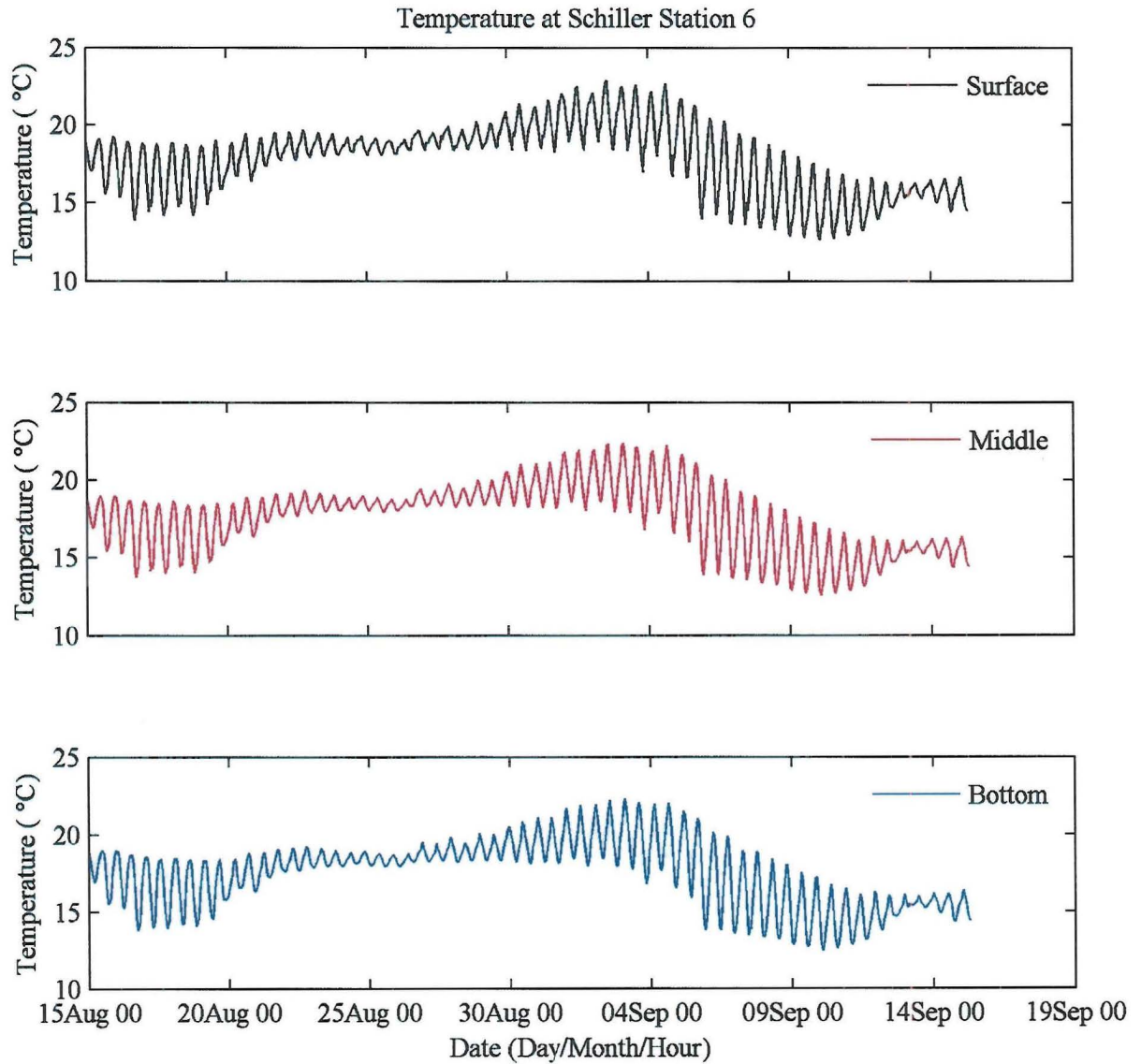
Figure 7. Plotted water temperature data recorded at locations A (surface), B (mid-depth) and C (bottom) at Station 6 for the Schiller Station thermal monitoring for the period 15 August through 15 September 2010.
