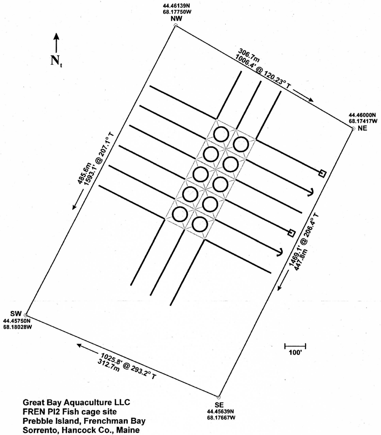
Figure 2. Cage system to be located on the FREN PI2 site
