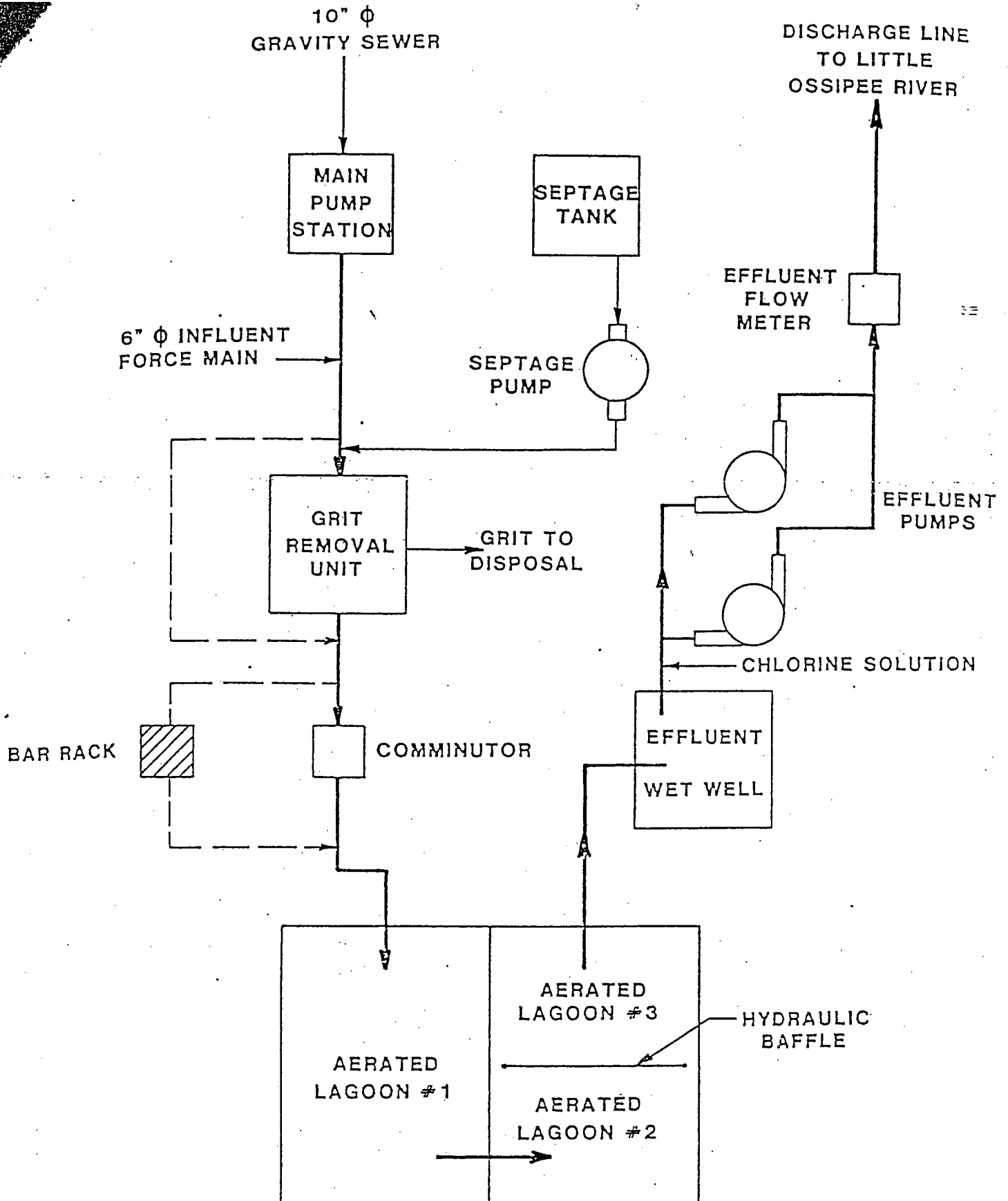
LIMERICK SEWERAGE DISTRICT PLANT FLOW SCHEMATIC FIGURE NO. 2
