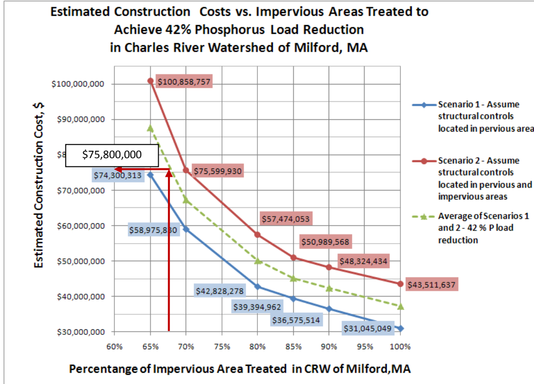
Figure 4.7: Estimated Capital Costs for Structural Controls to Achieve 42% Phosphorus Reduction for Milford (Implementation Scenario 3)
