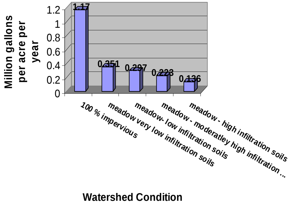
Annual Runoff Volume per Acre, Impervious vs. Pervious
