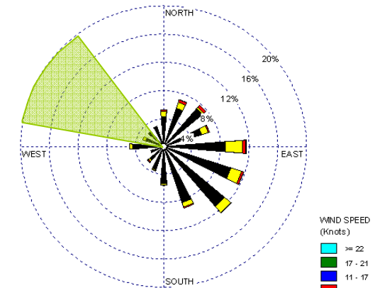
Vonore Middle School Composite Hourly Windrose Across Sampling Period (Sep. 4, 2009-Dec. 9, 2009)
