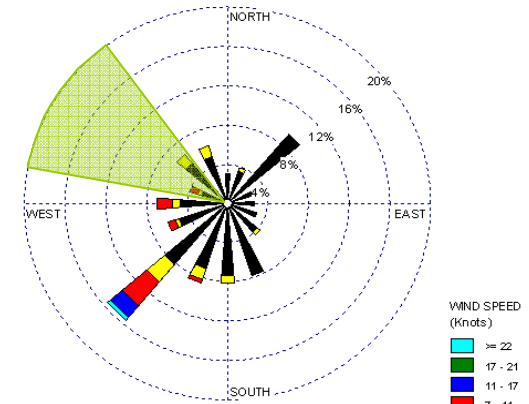
Vonore Middle School Composite Hourly Windrose on Sample Days (Sep. 4, 2009-Dec. 9, 2009)
