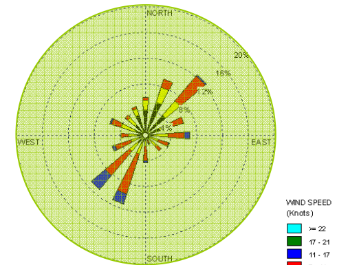
Spain Elementary School Composite Hourly Windrose Across Sampling Period (Aug. 17, 2009-Oct. 28, 2009)
