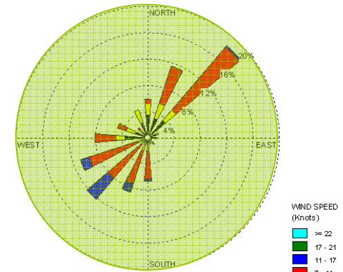
Spain Elementary School Composite Hourly Windrose on Sample Days (Aug. 17, 2009-Oct. 28, 2009)
