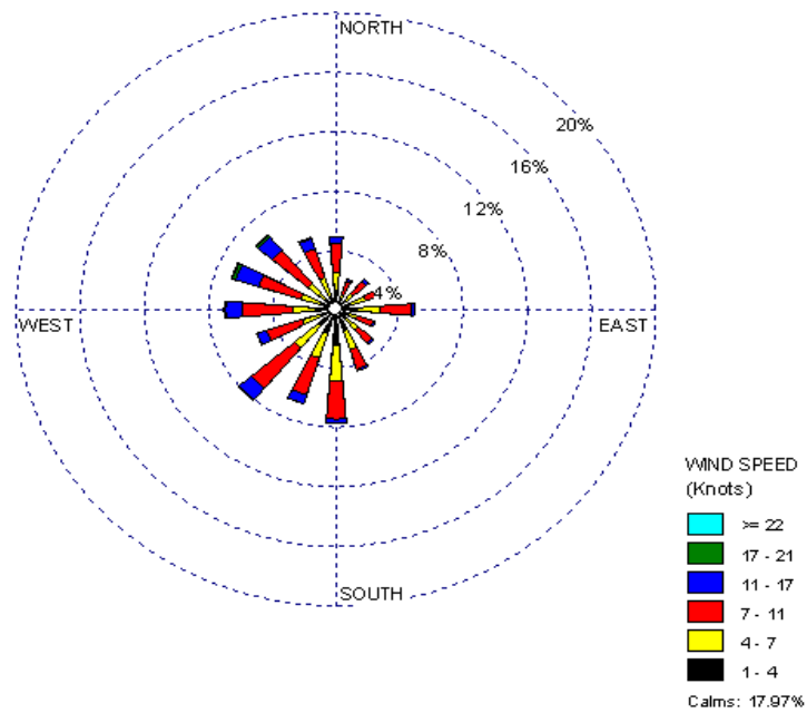
EAGLE CREEK AIRPARK AIRPORT NWS Station 2002-2007
