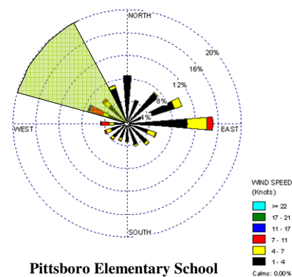
Pittsboro Elementary School Composite Hourly Windrose For Full Period (Aug. 23-Oct. 16, 2009)
