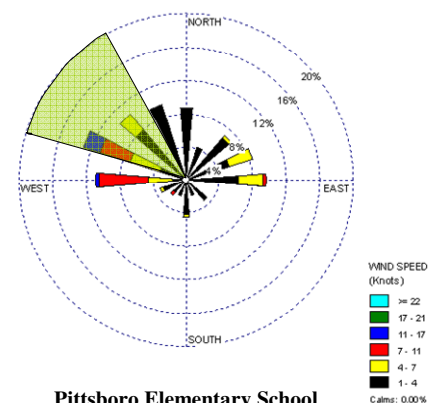
Pittsboro Elementary School Composite Hourly Windrose on Sample Days (Beginning Aug. 23-Oct. 16, 2009)
