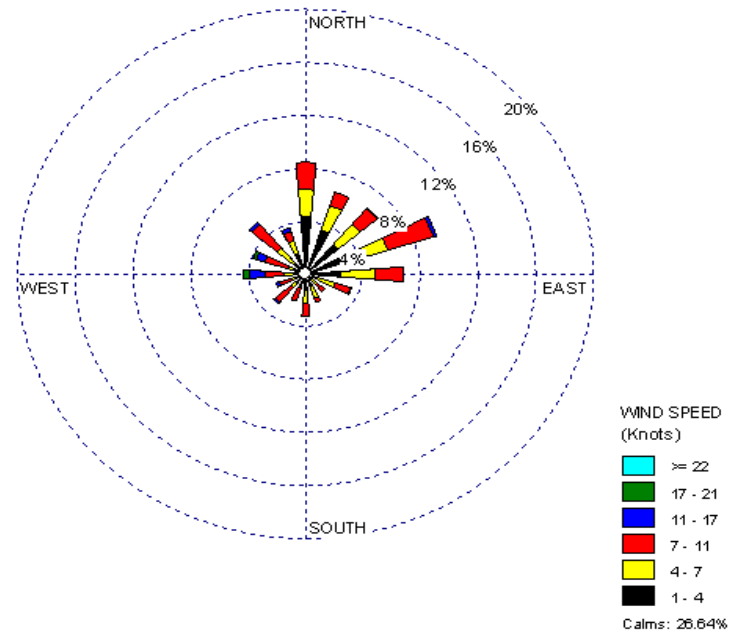
EAGLE CREEK AIRPARK AIRPORT NWS Station For Full Period (Aug. 23-Oct. 16, 2009) 1
