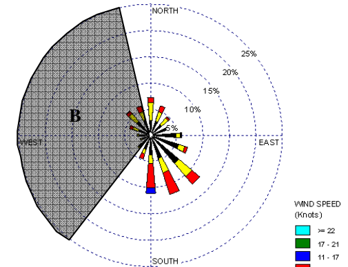
NW Harlee Elementary School Composite Hourly Windrose Across Sampling Period (Sep. 16, 2009-Dec. 15, 2009)
