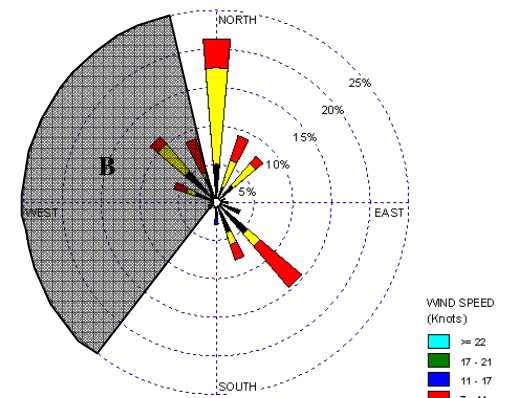
NW Harlee Elementary School Composite Hourly Windrose on Sample Days (Oct. 22, 2009-Dec. 15, 2009)
