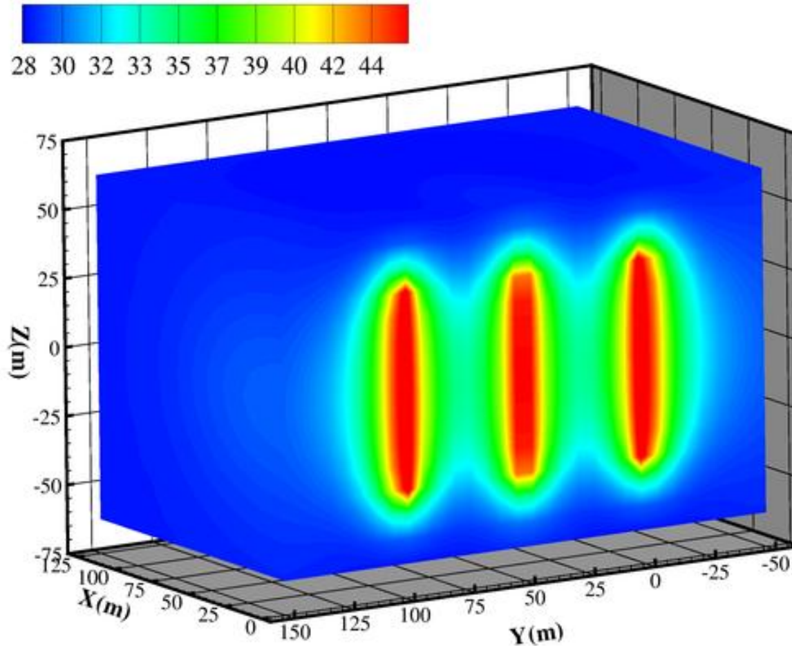
Distribution of pore pressures (MPa) in the formation after 3 hrs of injection
