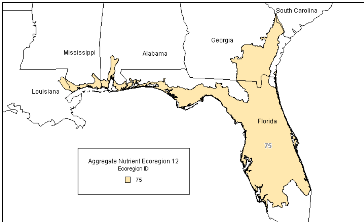
Figure 2. Ecoregion XII with level III subcoregion shown.
