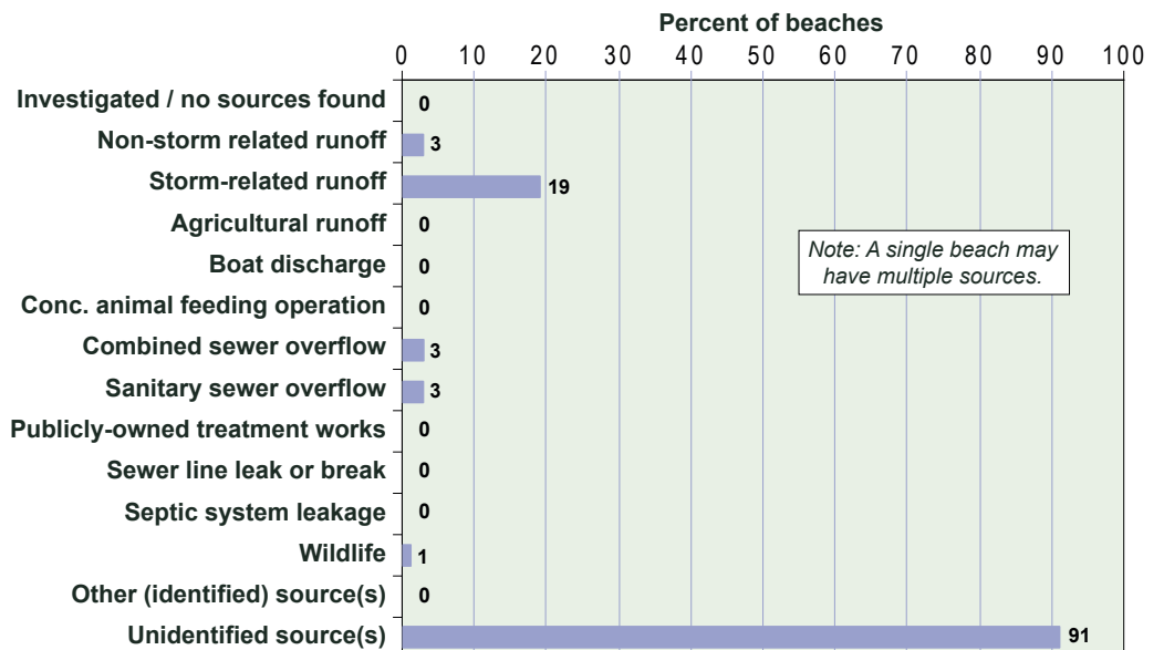
Figure 4: Percent of investigated monitored beaches affected by possible pollution sources (74 beaches).
