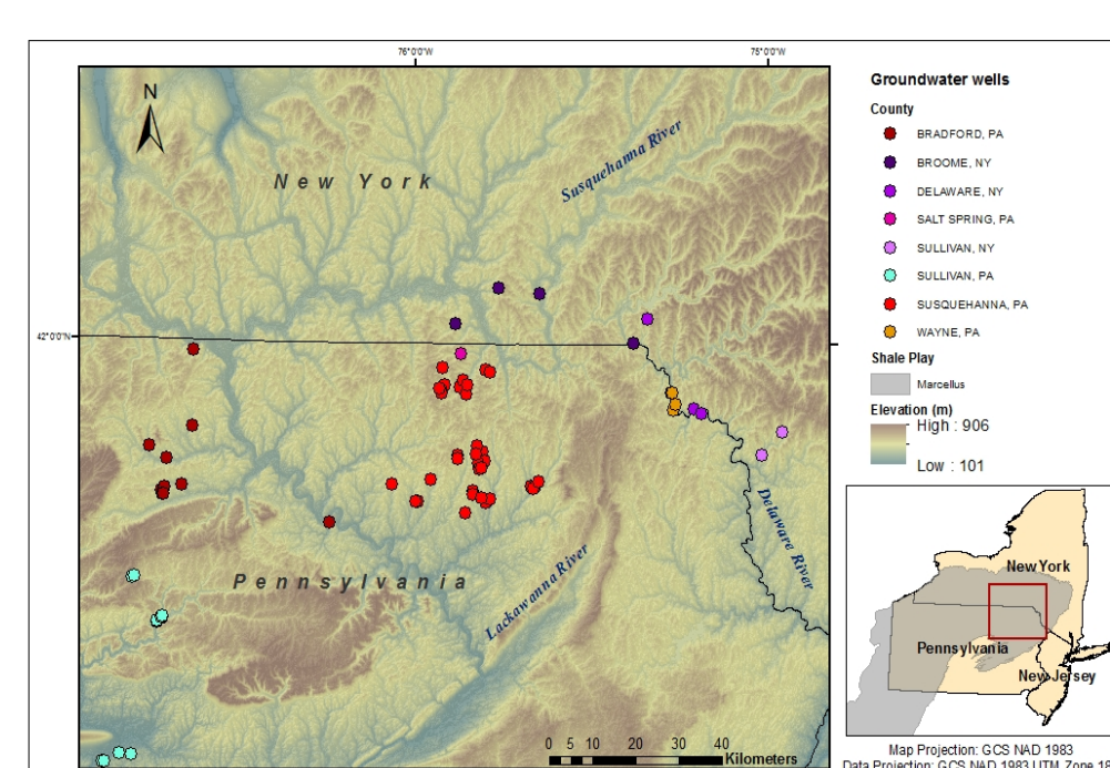
Figure 2: Digital elevation map of groundwater samples (n=72), sorted by location (county). Shaded brown areas represent higher elevations, while the blue-green demarks lower lying areas (valleys). All samples from this study were collected at distances >1km from active shale gas development at the time of sample collection across four counties in Pennsylvania (Bradford, Susquehanna, Wayne, Sullivan) and 3 counties (Delaware, Sullivan, Broome) in New York. Previous work identifies increasing [CH 4 ] and salt concentrations in valley bottoms (Warner et al, 2012, Molofsky et al, 2011).
