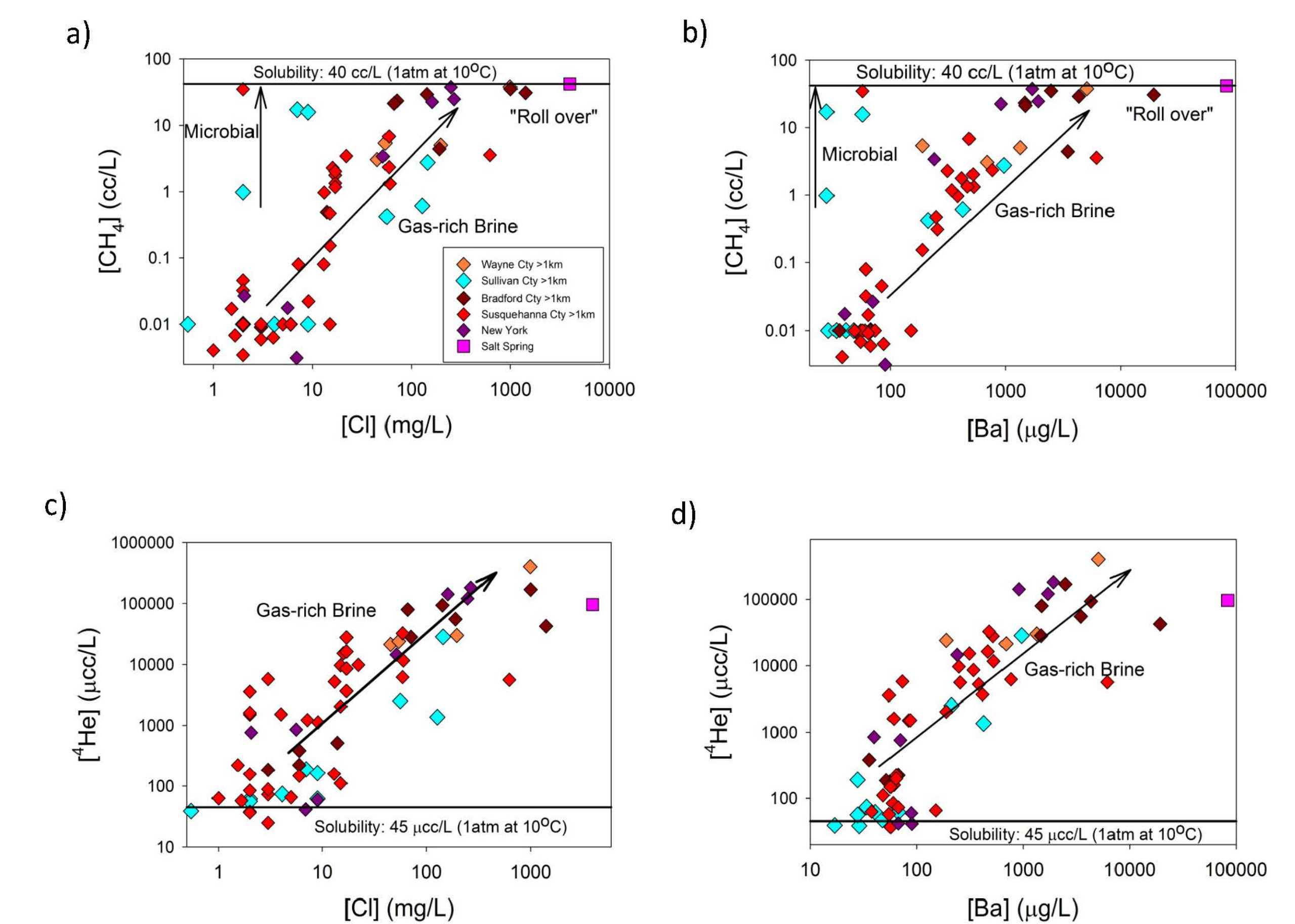
Figure 5: Variations of [Cl], [Ba], [CH 4 ], and [He] in groundwater and natural salt-rich spring located >1km from active shale gas drilling in Pennsylvania and New York. Sample colors indicate the county where samples were located. CH 4 and 4 He concentrations increase with Cl and Ba across the study area. The Cl-rich fluids contain elevated Br/Cl and Ba/Sr, as well as 87 Sr/ 86 Sr consistent with Middle Devonian Formation brines (i.e., Marcellus-type) (Warner et al, 2012). Notice that the increase in [CH 4 ] "rolls over" as methane concentrations approach saturation levels for shallow groundwater. The upper limit (solubility saturation = 40 cc/L at 1 atm) for [CH 4 ] demonstrates how groundwater solubility limits the maximum dissolved gas concentrations. The positive correlations of [ 4 He] with [Cl], [Ba], and [CH 4 ] suggests previous migration of a gas-rich, saline fluid from deeper formations into Upper Devonian aquifers across the region. The coexistence of CH 4 and [ 4 He] suggests a thermogenic source of methane.
