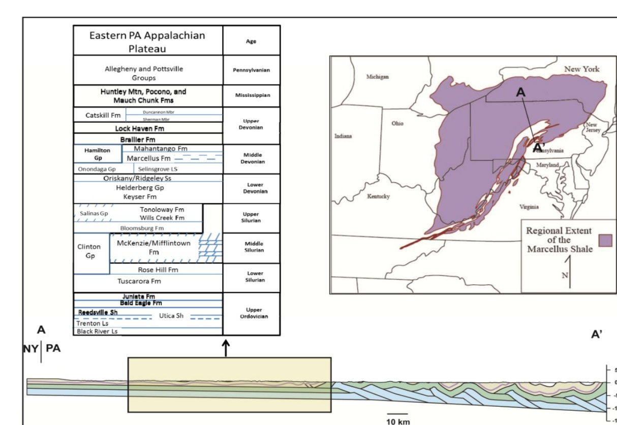
Figure 3: A generalized stratigraphic column (left), areal extent of the Marcellus Formation (right), and a simplified structural cross-section (reproduced from Sak et al, 2012) of the northern Appalachian Basin (NAB) plateau in northeastern PA and southeastern NY. The Marcellus Formation outcrop belt (upper right) is highlighted in red and the areal extent of the Marcellus Formation is shown in purple. The three principal shallow Upper Devonian aquifers include the Catskill, Lock Haven, and surficial alluvium. The generalized structural cross-section (bottom right) spans from the intensely deformed Valley and Ridge (southeast) to the Appalachian Plateau (to the north and west) across the Appalachian Structural Front (ASF). Samples in this study were collected within the yellow box at distances ranging from ~20-80km from the ASF.
