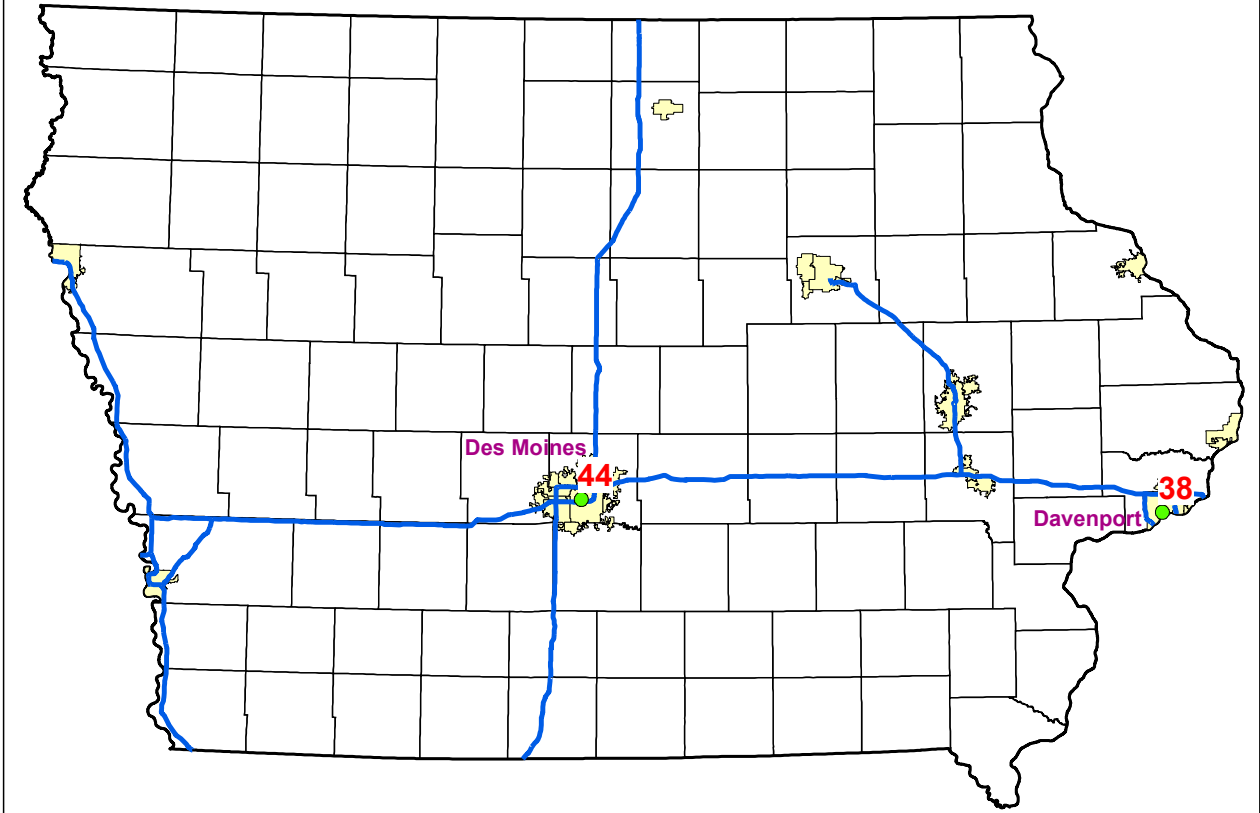
2008-2010 NO 2 One-Hour Design Values
