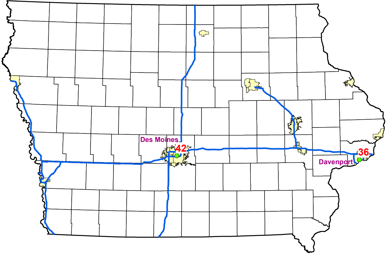
2010-2012 NO 2 One-Hour Design Values
