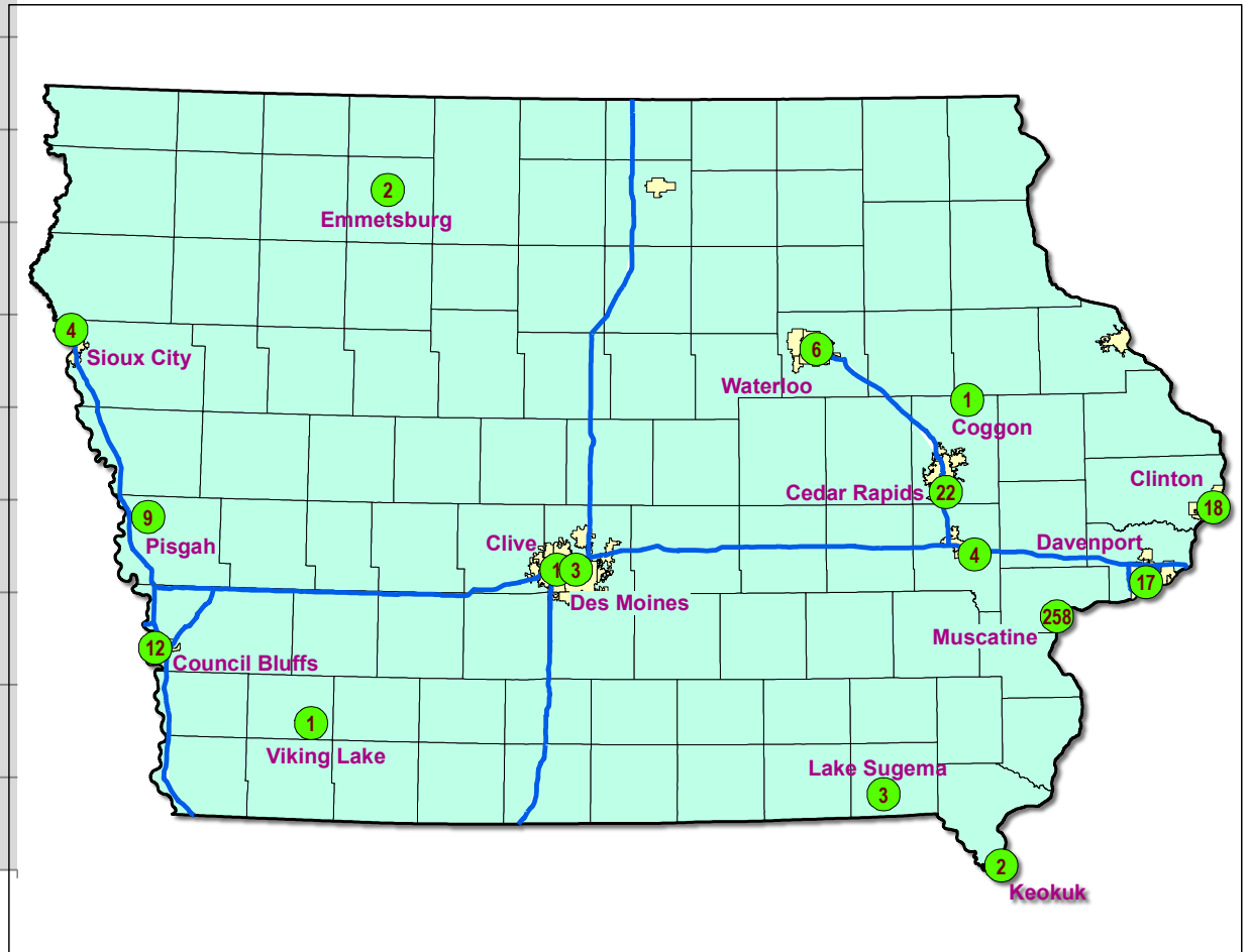
Location of NAAQS Exceedances: 2010-2014
