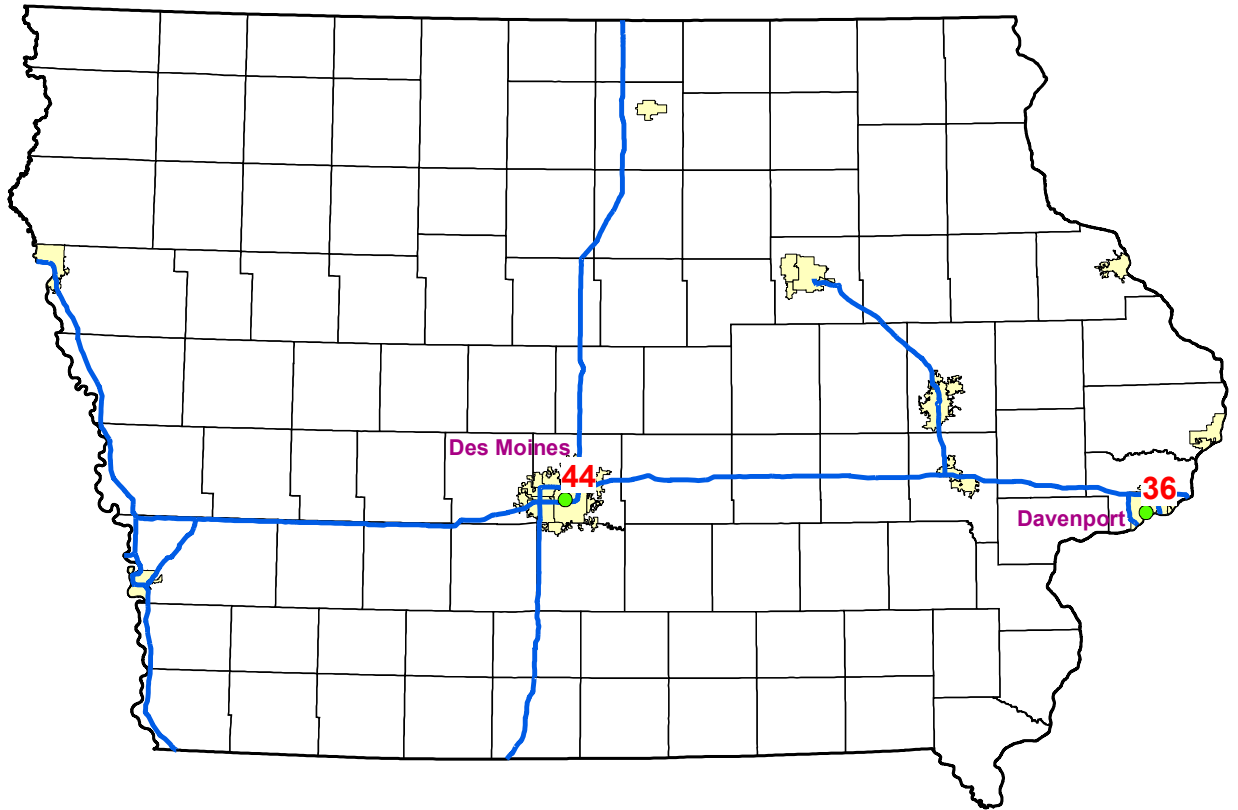
2009-2011 NO 2 One-Hour Design Values
