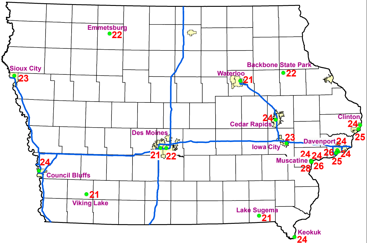
2011-2013 PM 2.5 24-Hour Design Values (µg/m 3 )
