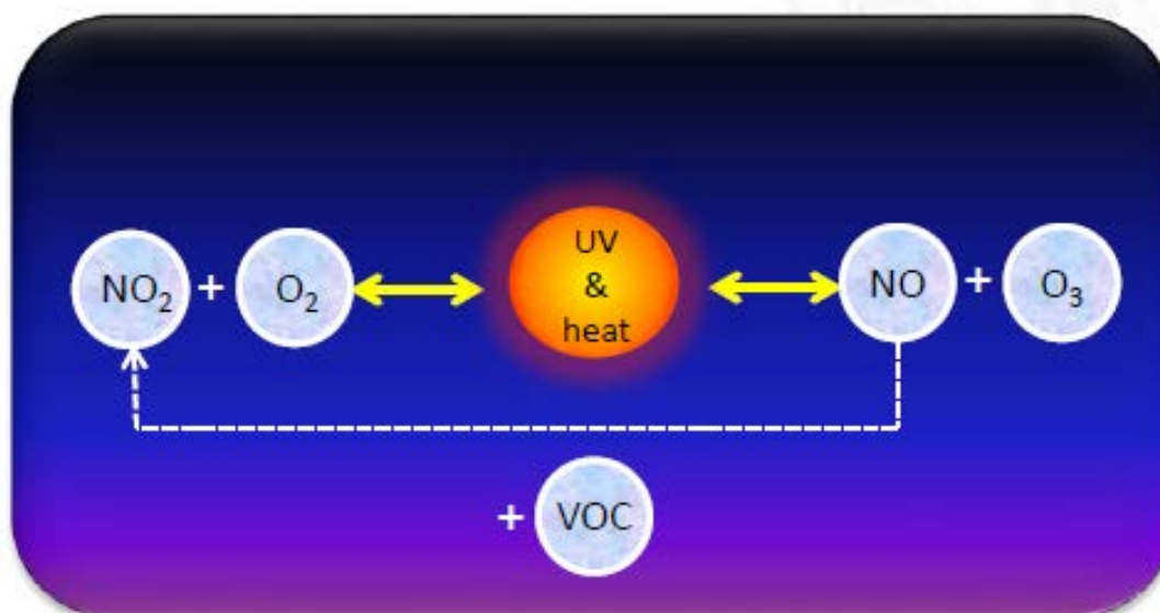
Figure 2-1 Ozone Formation
