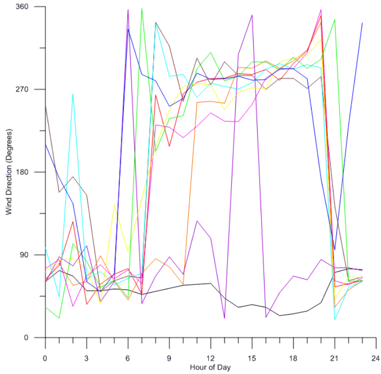
Figure 3-33 Average Diurnal Wind Pattern for 10 Highest Ozone Days at Queen Valley
