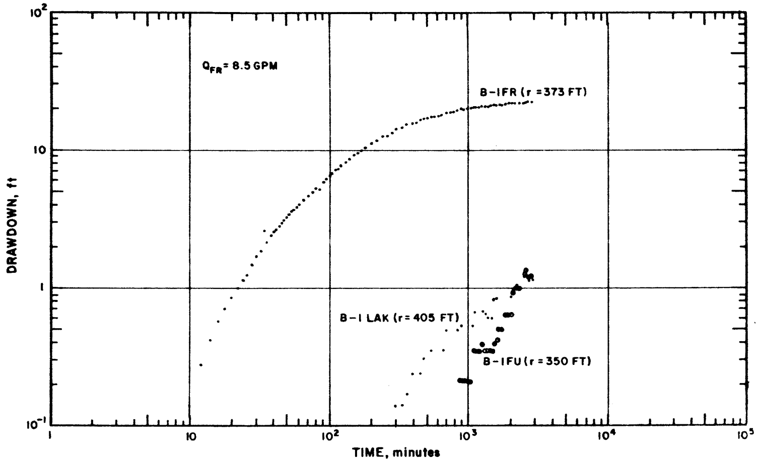
Figure 32: Logarithmic Graphs of Drawdown for B-1 Observation Well Group, Fall River Aquifer Test
