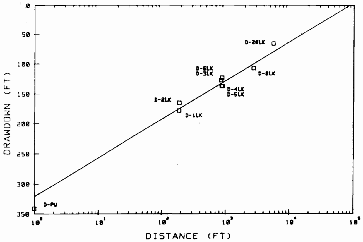
FIGURE 3. DISTANCE-DRAWDOWN GRAPH
