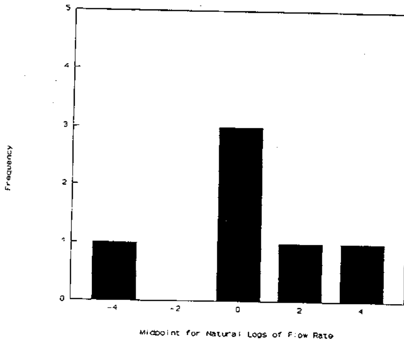
Figure A-2. Frequency Histogram for the Natural Logarithms of the Plastic Pipe Flow Rate Data
