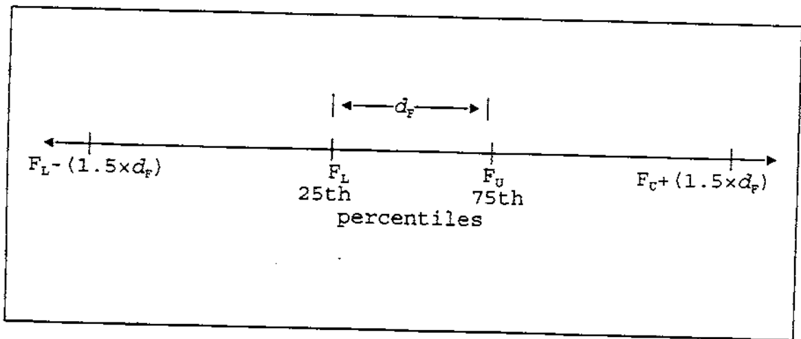
Figure A-3. Depiction of the Fourths ( F_L and F_U ), Fourth-Spread ( d_F ), and Boundaries ( F_L-1.5 \times d_F ; F_U+1.5 \times d_F ) for the F-Spread Outlier Detection Method
