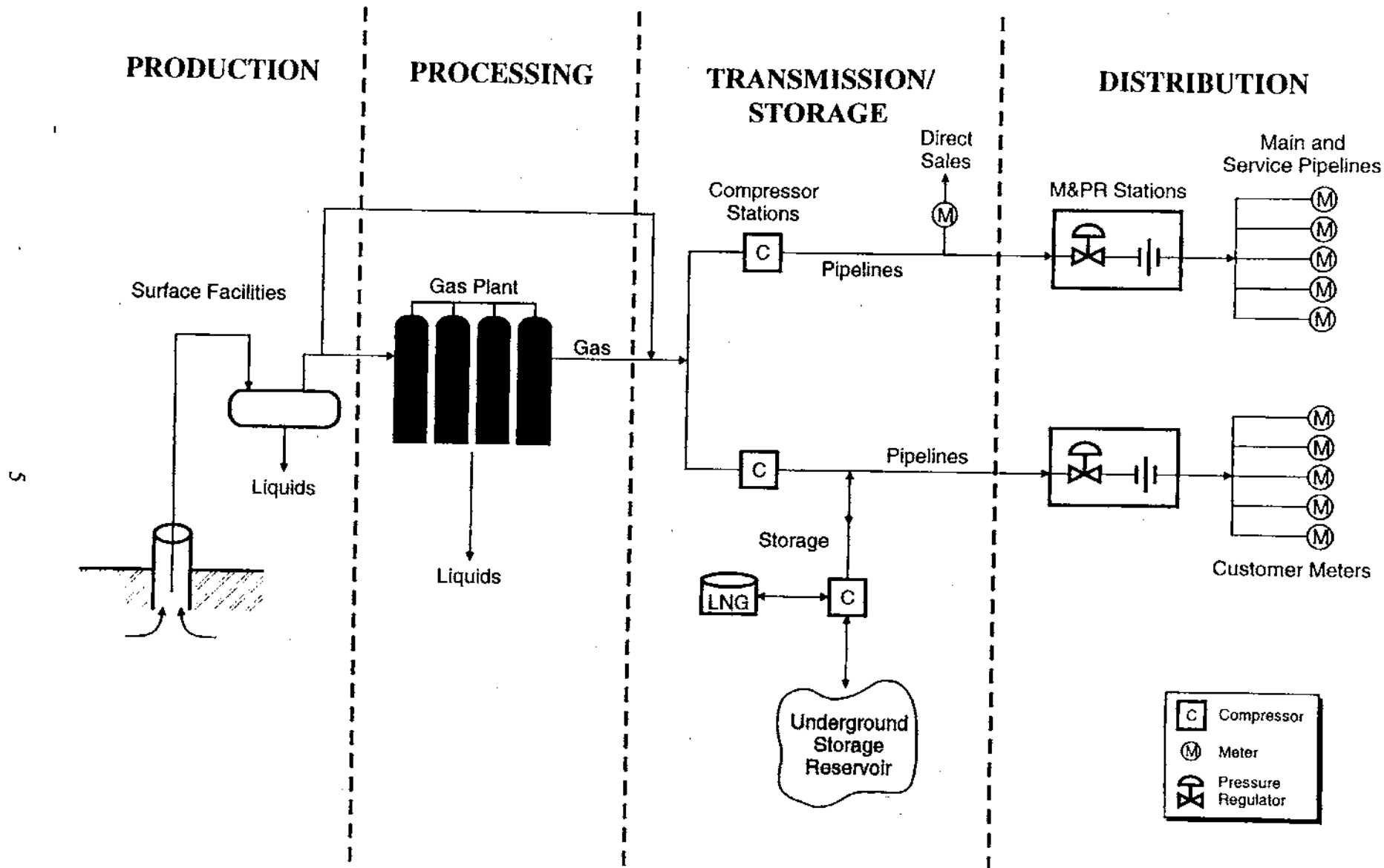
Figure 3-1. Gas Industry Flow Chart
