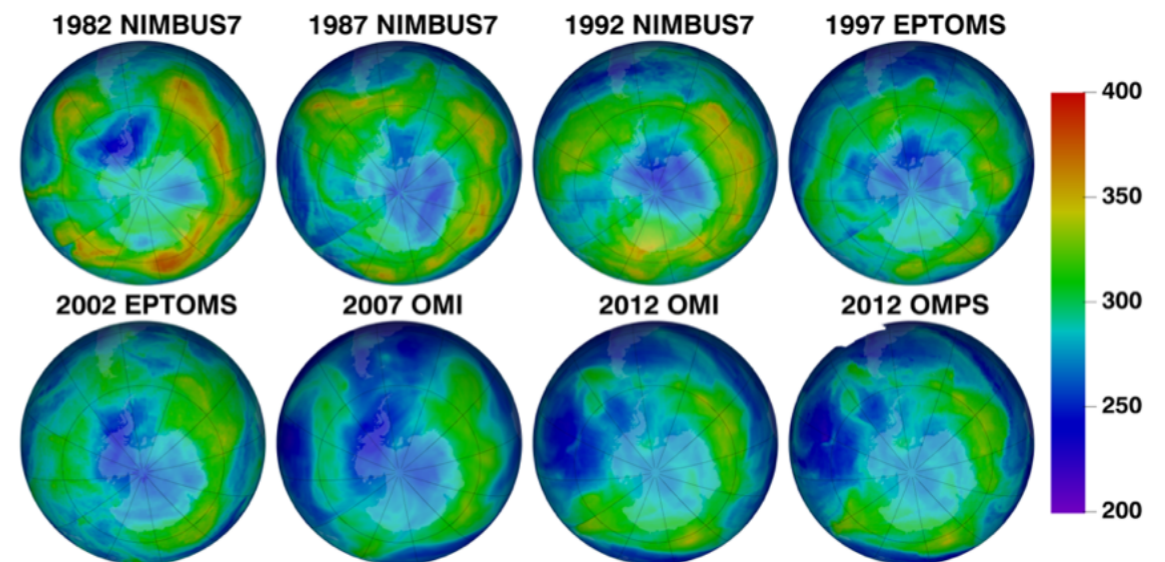
The above image shows the thickness of the Earth's ozone layer on January 27th from 1982 to 2012. This atmospheric layer protects Earth from dangerous levels of solar ultraviolet radiation. The thickness is measured in Dobson units, in this image, smaller amounts of overhead ozone are shown in blue, while larger amounts are shown in orange and yellow. Source: NASA/NOAA
