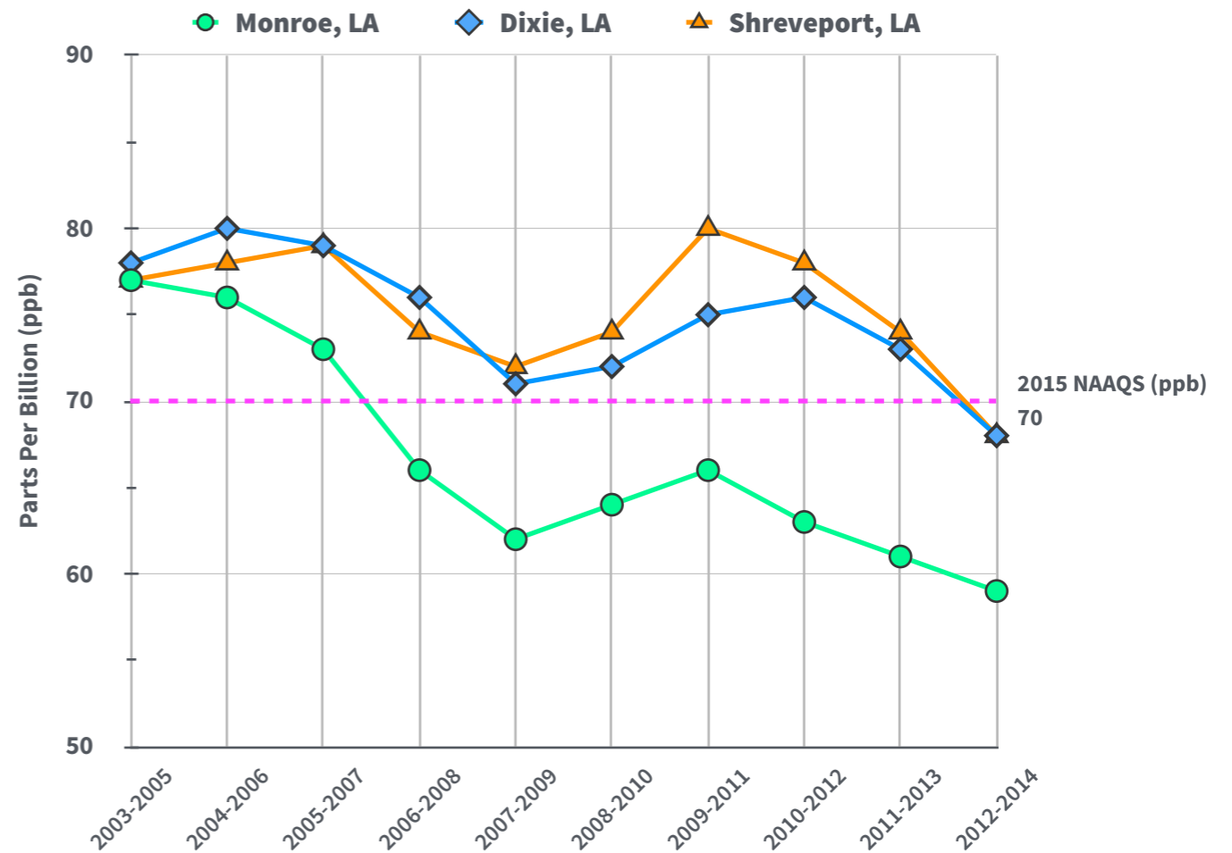
North Louisiana Air Monitor Trends 2003-2014 Monitor Level Design Values for the 8-Hour Ozone NAAQS
