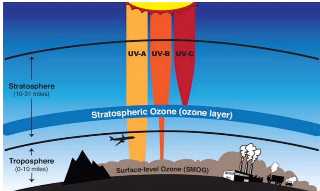
Miles above the surface of the Earth, a thin layer of ozone gas acts as a shield that protects us from harmful ultraviolet light. Source: NASA
