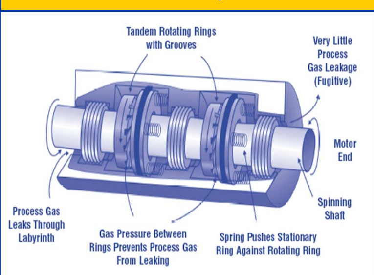
Exhibit 2b: Dry Seal
