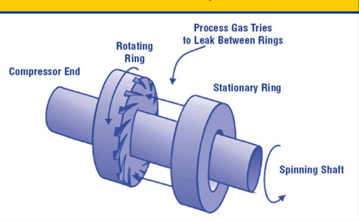
Exhibit 2a: Dry Seal
