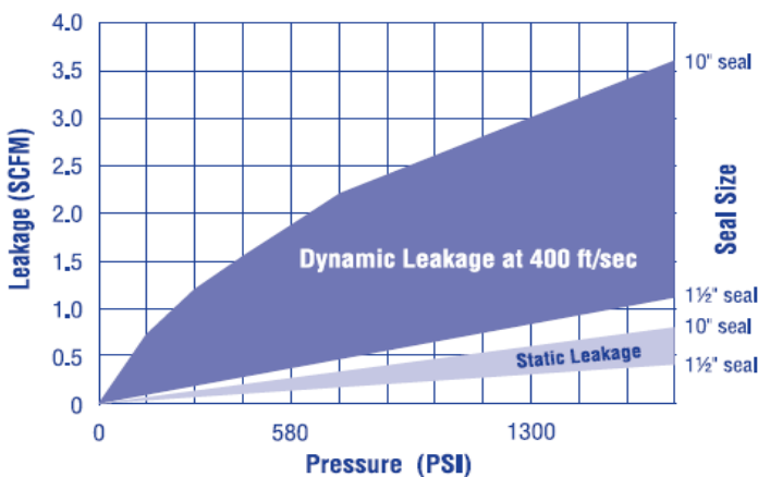
Exhibit 3: Dry Seal Performance Chart
