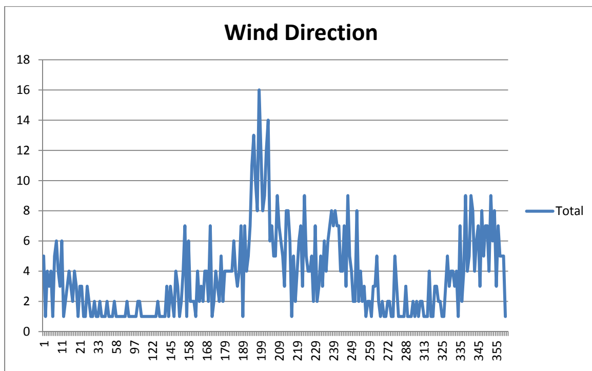
Figure 4 - Chart showing number of hits per degrees in Wind Direction, to depict areas of source influence
