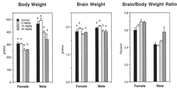
FIG. 4. Body and brain weight in adult rats exposed to PTU during preweaning development. Letters denote significant differences ( p < 0.05 ) between various treatment groups determined by Dunnett's multiple range test.
