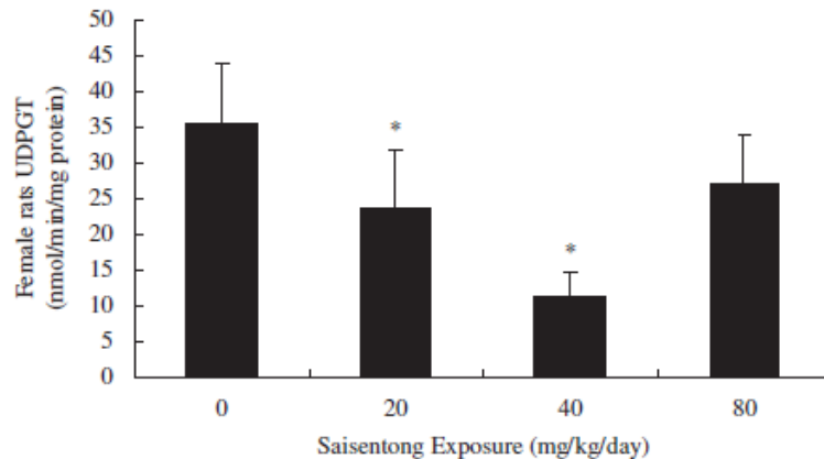
Fig. 3. Effect of pubertal exposure to Saisentong on liver microsomal enzyme, 4-nitrophenol uridinediphosphate-glucuronosyltransferase (UDPGT), activity in female rats. Data are presented as means \pm SE. *Denotes value significantly different from the control group at \alpha = 0.05 .
