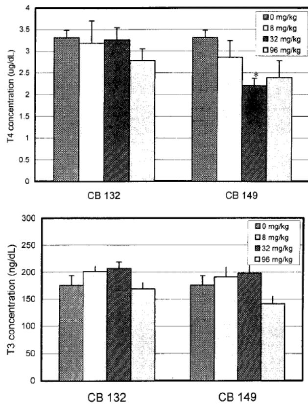
Fig. 1. Thyroid hormones status in prepubertal female rats administered CB 132 or CB149. *Significantly different from controls by Dunnett's t test ( p \leq 0.05 )
