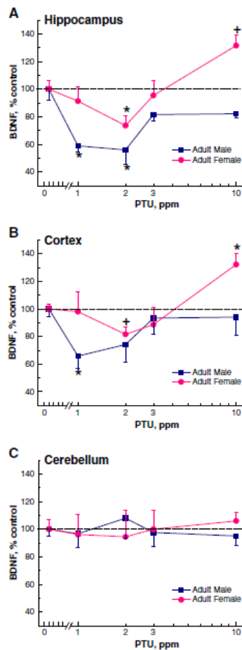
Fig. 5. Dose-effect relationships for BDNF protein expression and PTU dose in adult male and female offspring in each brain region. BDNF values are normalized to the 0 ppm value (= 100) for the respective gender in that brain area. Values are expressed as mean \pm SEM in percent control with N=5-11 for each PTU dose in each gender; *p<0.05 compared to the 0 ppm value of the same gender. Marginal effects seen in female hippocampus at 10 ppm and cortex at 2 ppm are depicted as +p<0.06 when contrasted to 0 ppm value in females.
