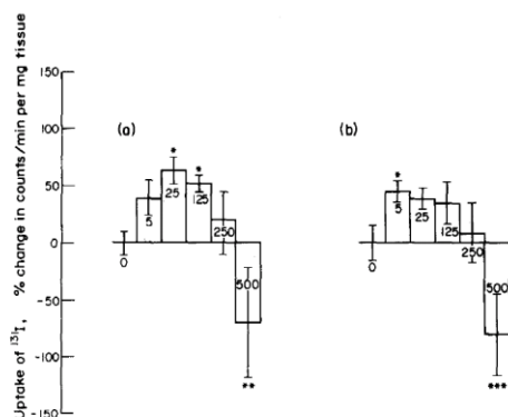
Fig. 2. Mean uptake of ^{131}\text{I} by the thyroids of groups of five male rats fed 0–500 ppm ETU for (a) 18 or (b) 24 months. Vertical bars represent the SEM and asterisks indicate results differing significantly from the control: * P < 0.05 ; ** P < 0.01 ; *** P < 0.001 .
