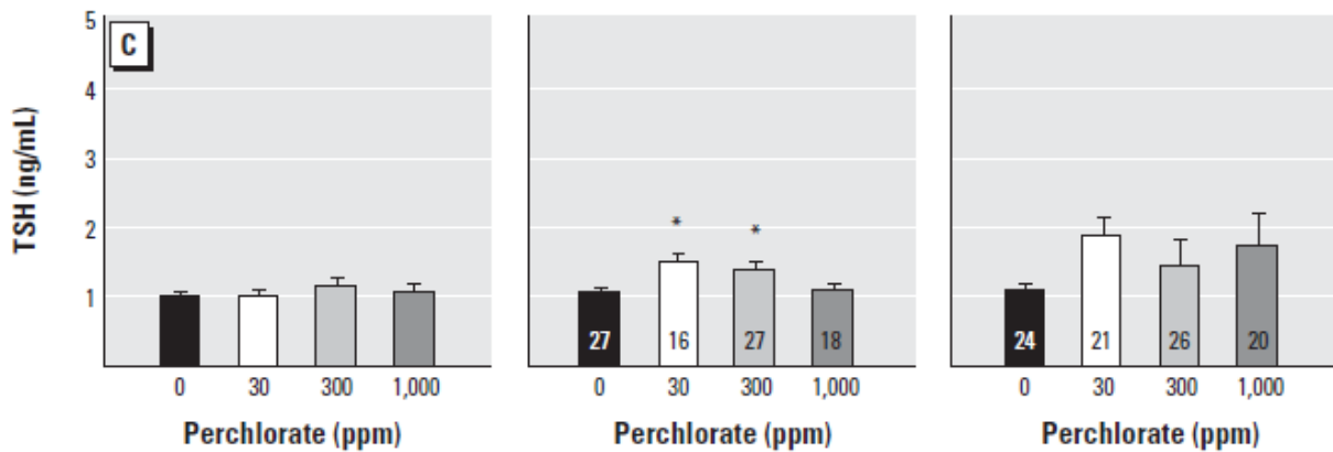
Figure 3. Thyroid hormone concentrations (mean ± SE) in pups exposed to perchlorate beginning on GD6 and sacrificed on PNDs 4, 14, or 21. (A) T 3 . (B) T 4 . (C) TSH. Data from PND4 represent males and females because samples were pooled to provide sufficient serum for the assays. No differences in serum hormones were detected between sexes on PND14 and PND21 ( p > 0.05 ), so data were collapsed across, and mean value per litter at each age was analyzed. Numbers within the bars represent sample sizes. * p < 0.05 by Dunnett's t .
