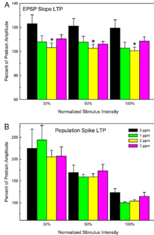
FIG. 6. Individual animal normalization to detect LTP magnitude differences across dose groups. To simplify detection of dose-dependent differences in LTP, the percent increase above pretrain amplitudes was calculated for EPSP slope and PS based on the intensity that produced a PS 30, 50, and 100% of maximal for each individual animal in the pretrain baseline I/O function. This analysis confirmed significant reductions in EPSP slope at all dose levels when collapsed across intensities (A), consistent with the pattern portrayed in Figure 5. Mean contrasts tests at each intensity suggested greater decrements in the 2 ppm dose group. (B) Greater LTP magnitude was seen at lower intensities for PS, but no effect of PTU was evident. Tukey's t -test * p < 0.05 LTP of the PS was not affected by PTU (B).
