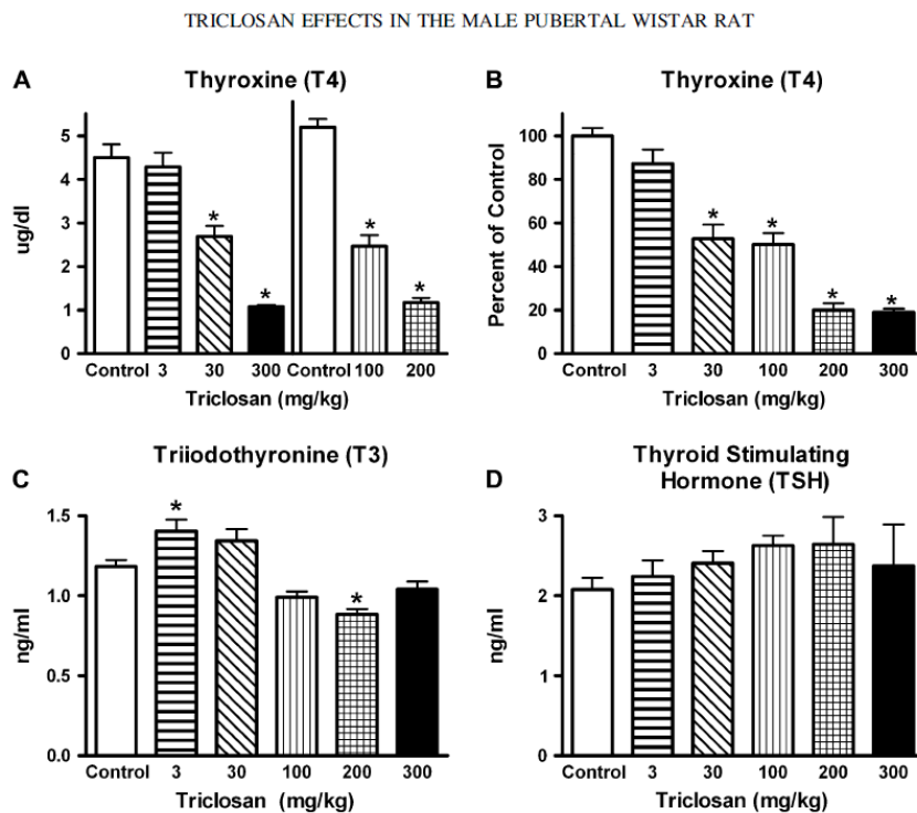
FIG. 6. The effect of a 31-day exposure to triclosan (mg/kg/day) on (A) mean total serum T4, (B) mean total T4 shown as percent of control, (C) mean total T3, and (D) mean serum TSH concentrations in the male Wistar rat. * p < 0.05 as compared with control mean.
