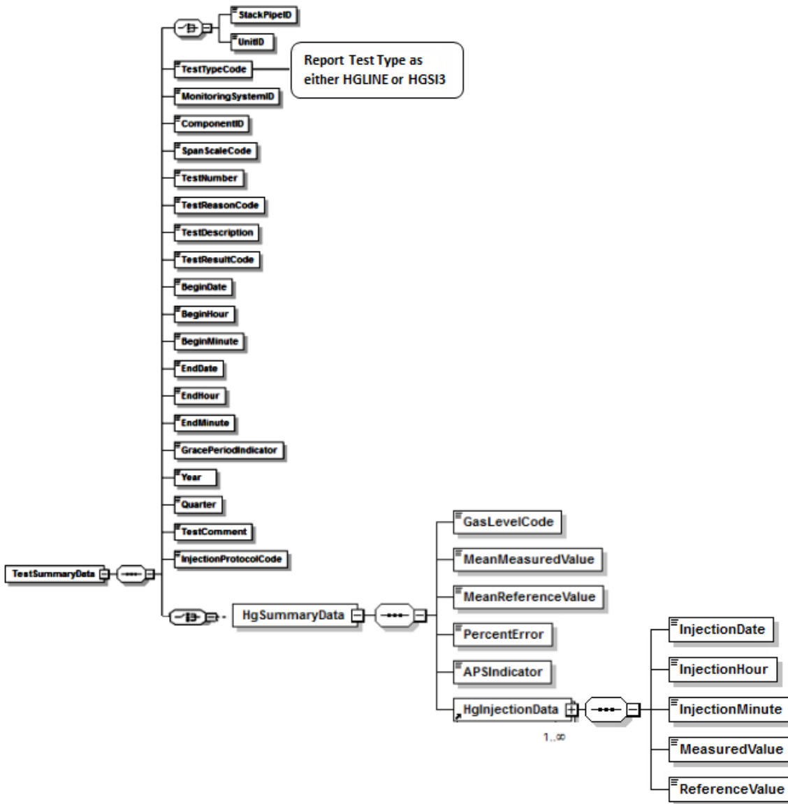
Figure 13: Hg Linearity/System Integrity Check XML Elements
