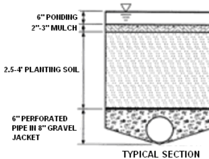
Figure 2-5. Typical cross sections for biofiltration.
