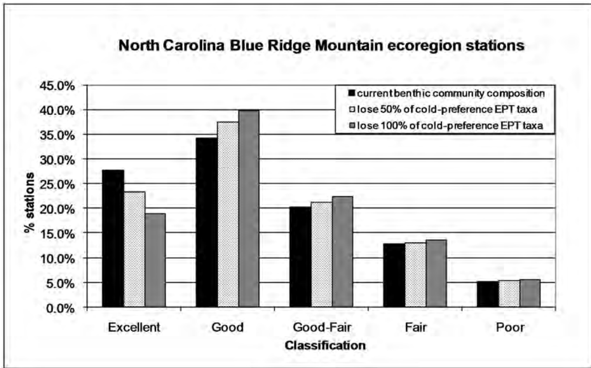
Figure 3-2 Example of how reference station status can degrade over time due to climate-induced increases in stream temperature.
