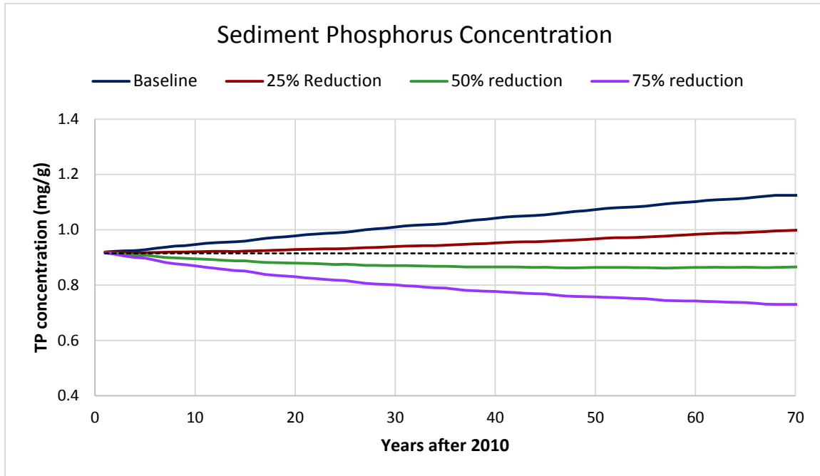
Figure 3: Average annual bay-wide sediment T P concentration
