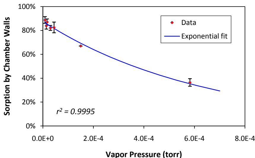
Figure 6.49. Experimental results and exponential fit for sorption of PCB congeners by the interior walls of the 53-L chamber as a function of vapor pressure (error bar = \pm 1 SD)
