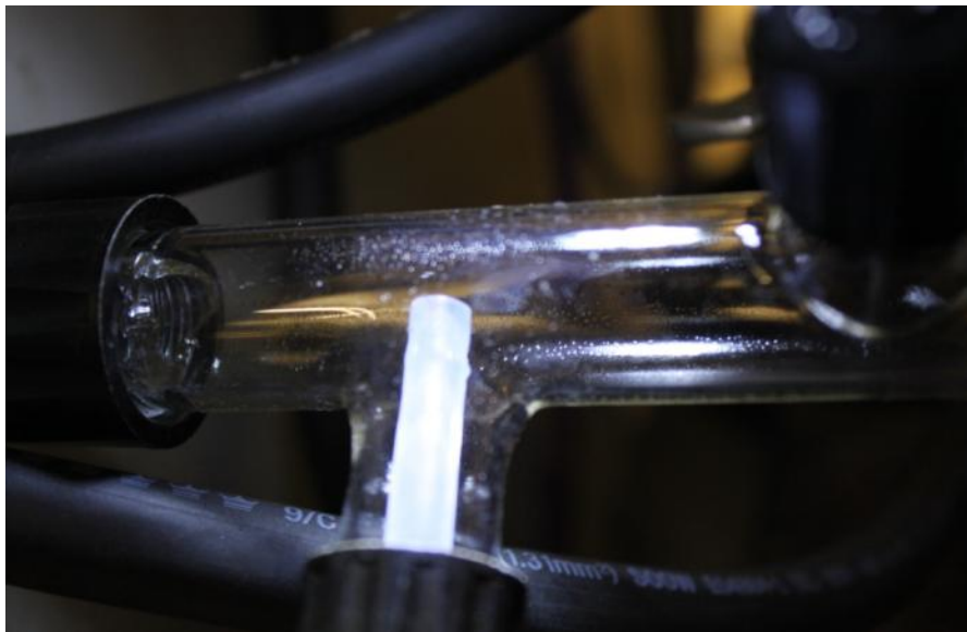
Figure E.6. Condensation of fluids in the chamber outlet manifold after the failure of the light ballast
