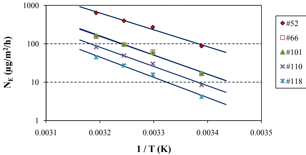
Figure 4.9. Normalized emission factor ( N_E ) as a function of temperature for five congeners in caulk sample CK-13 (trend lines for congeners #66 and #101 are superimposed)
