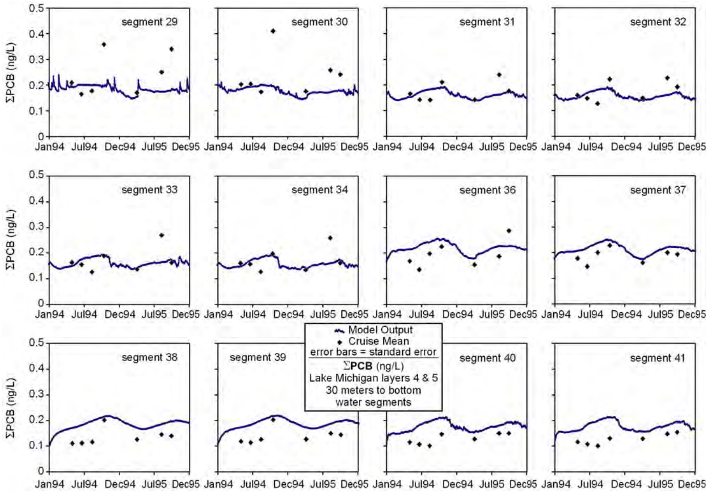
Figure 4.5.7. Temporal profiles of \Sigma\text{PCBs} (dissolved phase + particulate phase) in Lake Michigan water column segments for PCB dynamics calibration of the LM2-Toxic and the LMMBP cruise mean data (Continued).
