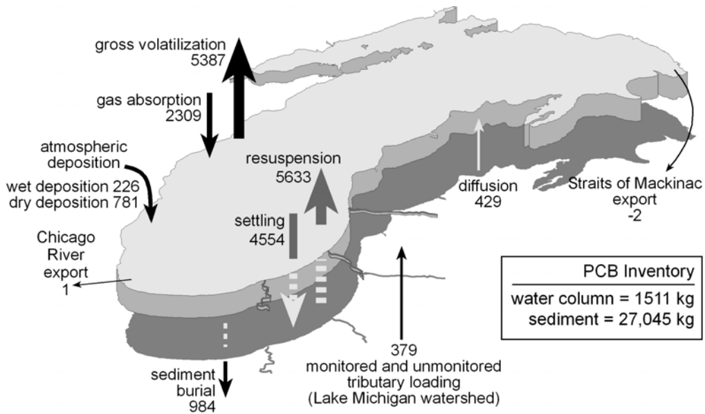
Figure 3.3.22. MICHTOX predicted mass balance fluxes and inventories (kg/year) for 1994-1995, whole lake results.
