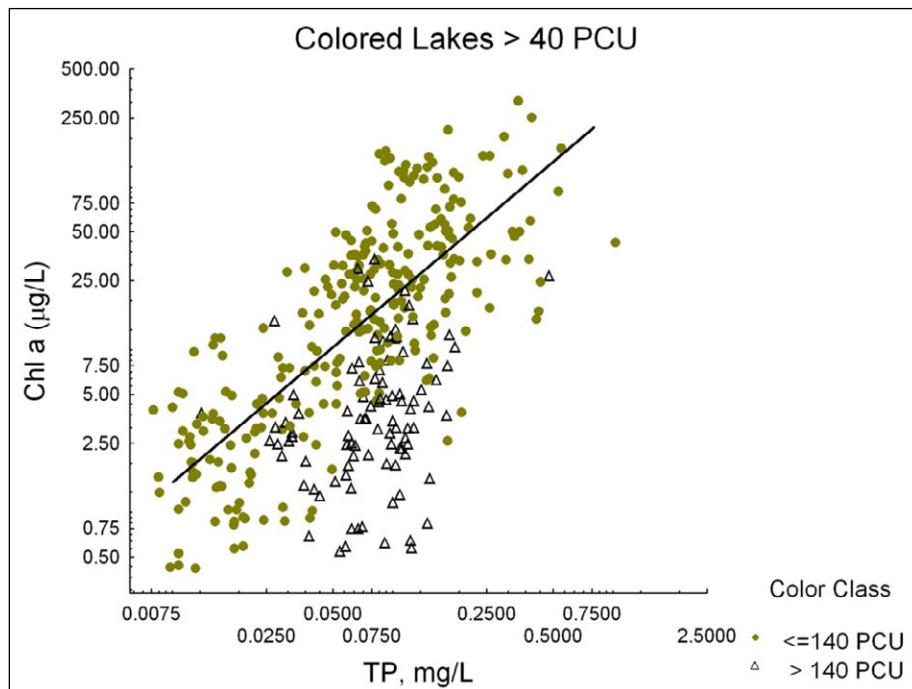
Figure 2-24. Chl-a – TP regression in intermediate colored lakes. Note that symbols are as in Figure 2-23.
