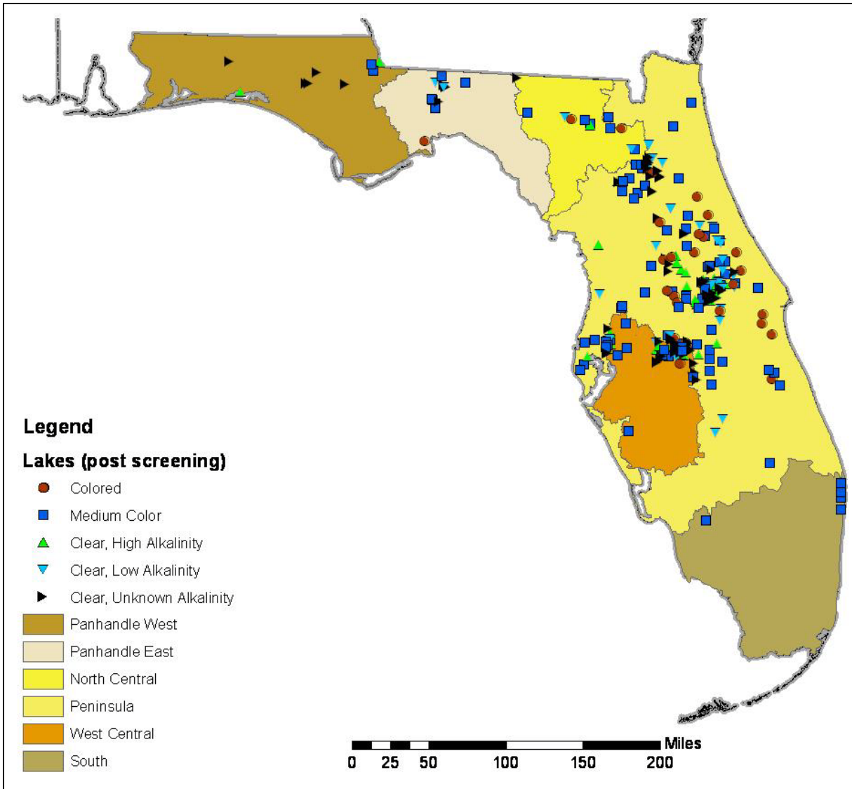
Figure 2-14. Distribution of Florida lakes by color and alkalinity class after data screening. Data screening methods are described in Section 2.2.2. EPA's stream Nutrient Watershed Regions (NWRs) are shown for geographical reference. See Chapter 1 for more information on stream NWRs.
