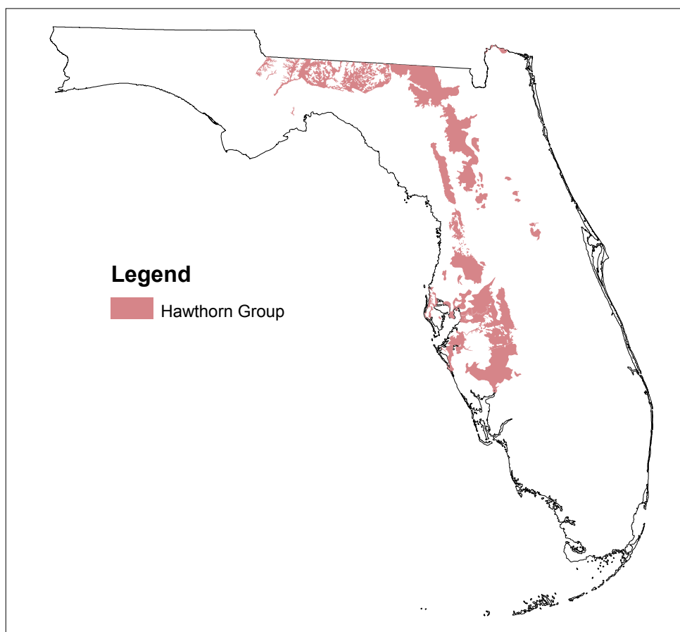
Figure 1-3. Map of Hawthorn Group in Florida, indicating major phosphatic regions.
