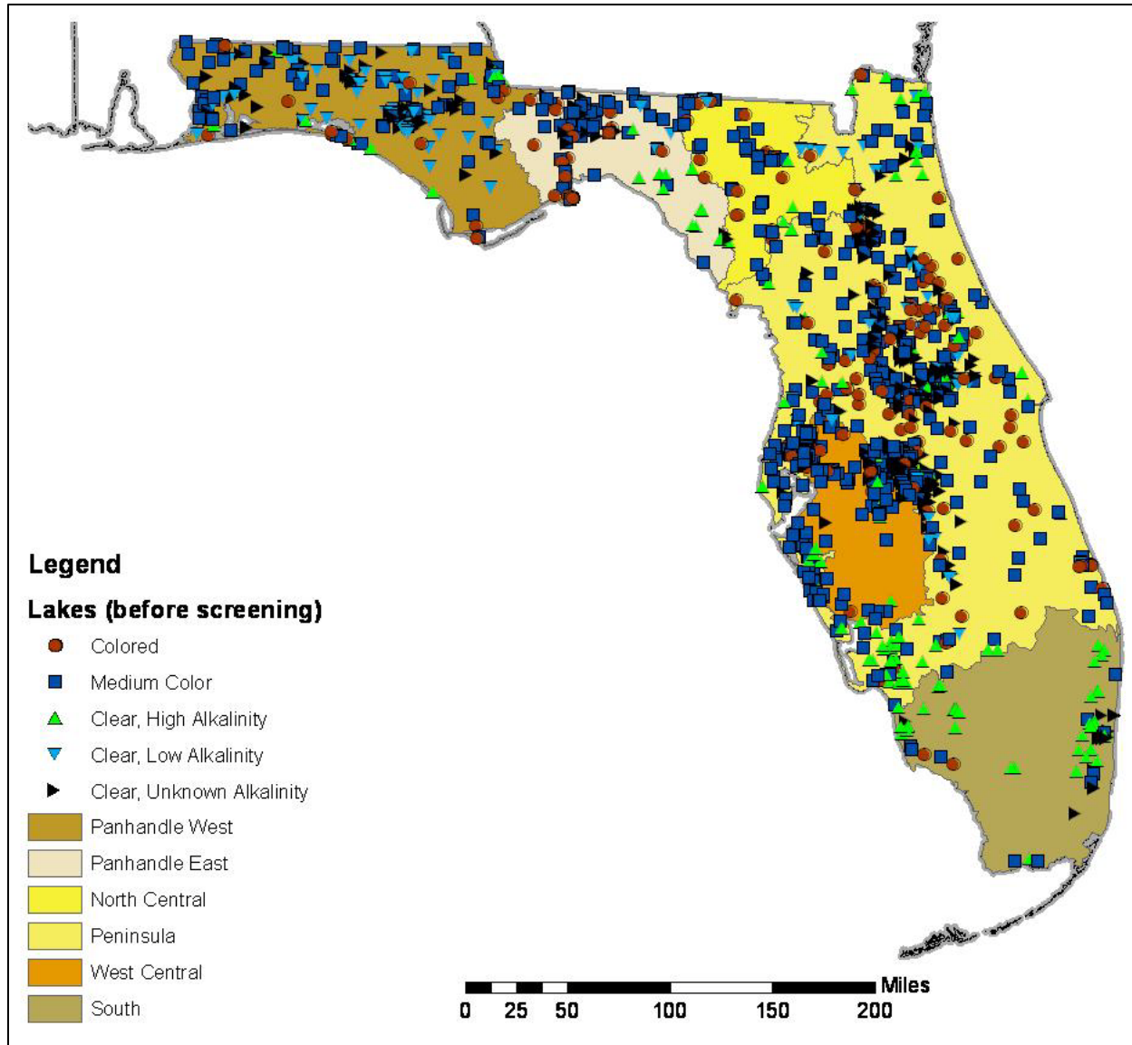
Figure 2-13. Distribution of Florida lakes by color and alkalinity class before data screening. Data screening methods are described in Section 2.2.2. EPA's stream Nutrient Watershed Regions (NWRs) are shown for geographical reference. See Chapter 1 for more information on stream NWRs.
