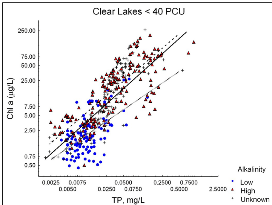
Figure 2-22. Chl-a – TP regressions for clear lakes. Note that symbols are as in Figure 2-21.
