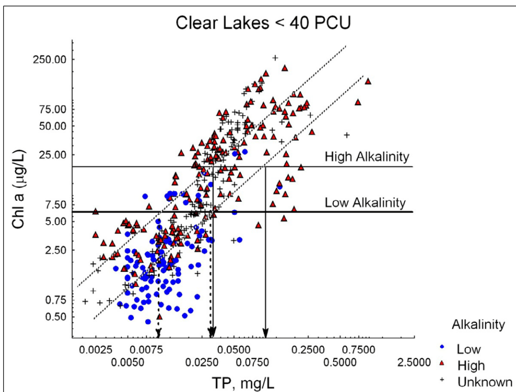
Figure 2-31. Chl-a and TP in clear lakes, showing 50% prediction interval (dotted lines). Note that symbols and data as in Figure 2-21. High alkalinity: chl-a criterion (20 µg/L) for high alkalinity lakes; low alkalinity: chl-a criterion (6 µg/L) for clear, low alkalinity lakes. Solid arrows: criteria range for high alkalinity lakes; dashed arrows: criteria range for clear, low alkalinity lakes.
