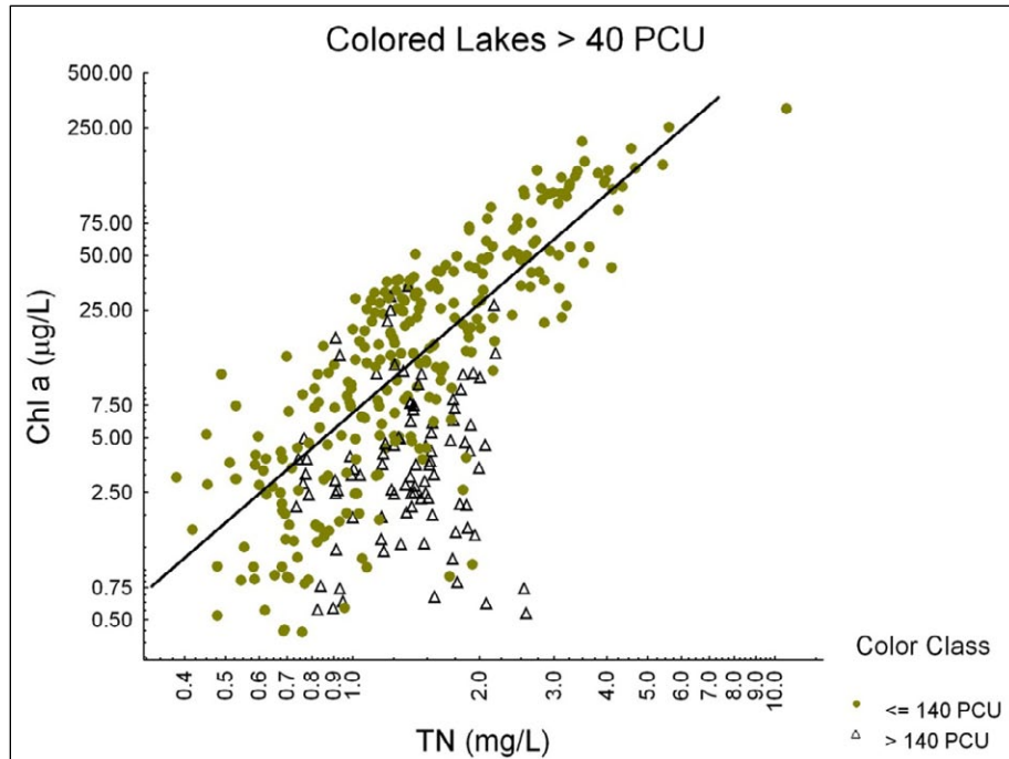
Figure 2-23. Chl-a – TN regression in intermediate colored lakes. Note that closed circles: intermediate color lakes; open triangles: high color lakes. Regression line is for medium colored lakes; high color lakes NS.
