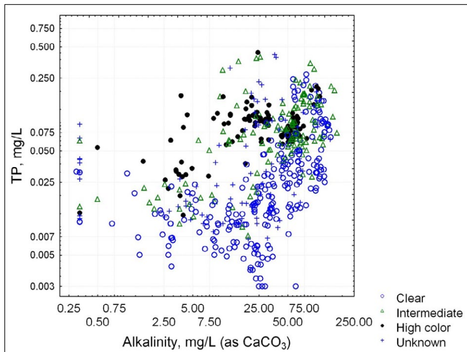
Figure 2-8. Scatter plot of TP and alkalinity in Florida lakes, annual geometric means.
