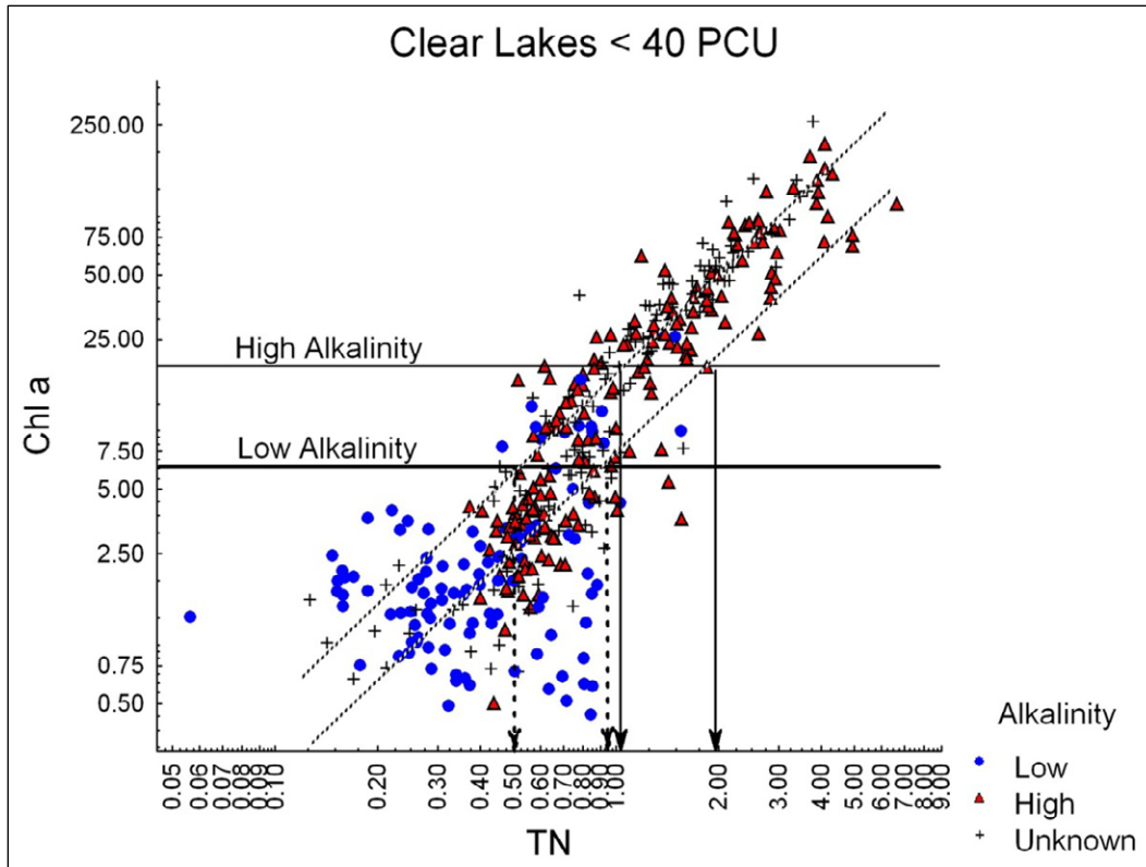
Figure 2-30. Chl-a and TN in clear lakes, showing 50% prediction interval (dotted lines). Note that symbols and data as in Figure 2-21. High alkalinity: chl-a criterion (20 µg/L) for clear, high alkalinity lakes; low alkalinity: chl-a criterion (6 µg/L) for clear, low alkalinity lakes. Solid arrows: criteria range for high alkalinity lakes; dashed arrows: criteria range for clear, low alkalinity lakes.
