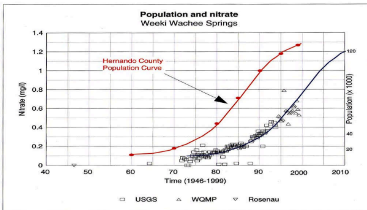
Figure 3-1. Changes in NO 3 concentration in Weeki Wachee Spring discharge and population of Hernando County, Florida.
