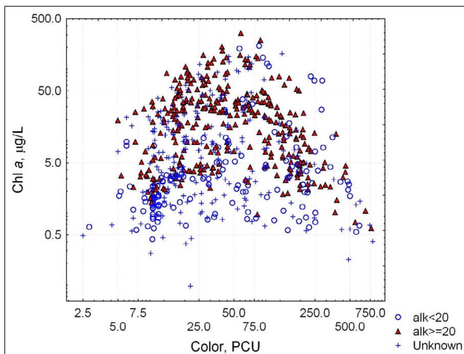
Figure 2-12. Scatter plot of chl-a and color in Florida lakes, annual geometric means for different lake alkalinity classes.
