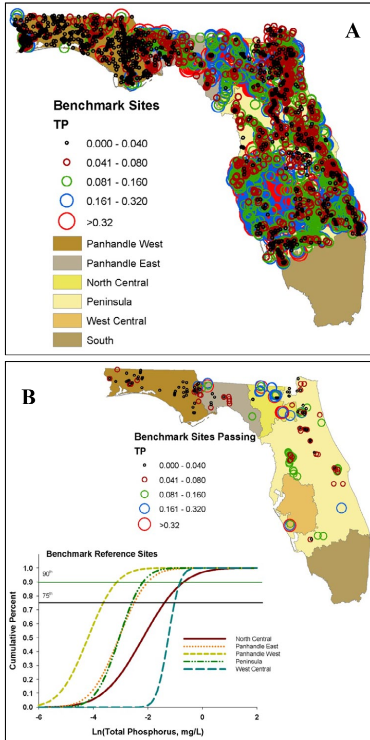
Figure 1-19. Plot of TP concentrations among benchmark reference sites across EPA's NWRs for the Benchmark Population before (A) and after (B) screening. Note that concentrations graphed are Ln(TP, mg/L). Also shown (in B) are cumulative percent frequencies of TP concentrations at benchmark sites.
