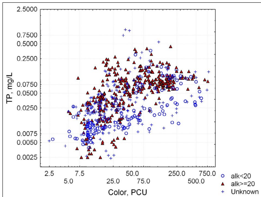
Figure 2-11. Scatter plot of TP and color in Florida lakes, annual geometric means for different lake alkalinity classes.
