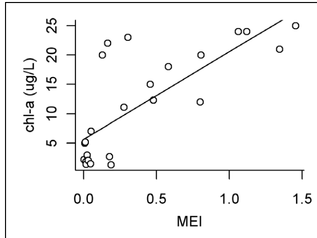
Figure 2-19. MEI versus chl-a in calibration data set (from Lowe et al. 2009). Note that the straight line is the simple linear regression fit; lake color did not contribute significantly to the model.
