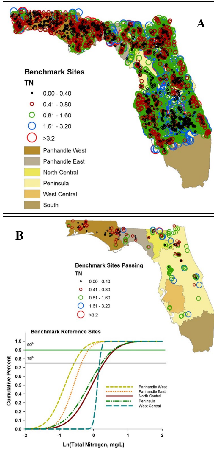
Figure 1-15. Plot of TN concentrations among benchmark reference sites across EPA's NWRs for the Benchmark Population before (A) and after (B) screening. Note that concentrations graphed are Ln(TN, mg/L). Also shown (in B) are cumulative percent frequencies of TN concentrations at benchmark sites.
