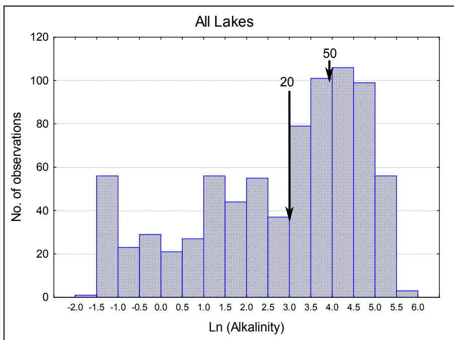
Figure 2-6. Distribution of average log alkalinity in Florida lakes (natural log scale). Note that alkalinities of 20 and 50 mg/L shown by arrows; alkalinities are means of annual means for the period of record for each lake; N = 739 lakes.
