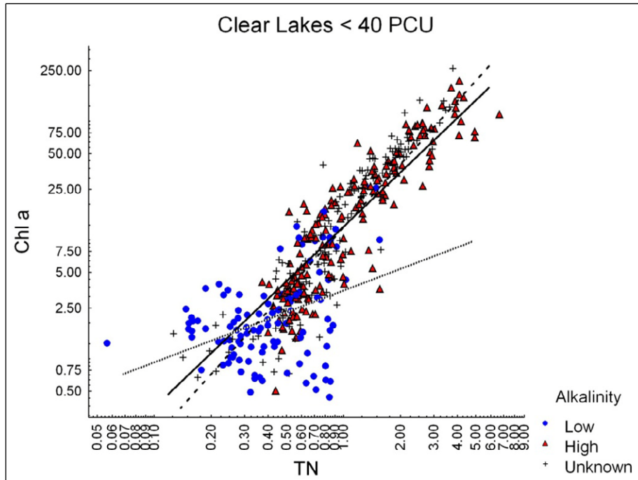
Figure 2-21. Chl-a – TN regressions for clear lakes. Note that triangles: high alkalinity; closed circles: low alkalinity; crosses: unknown. Dotted line: low alkalinity regression line; dashed line: high alkalinity regression; solid line: all clear lakes. Annual geometric means.
