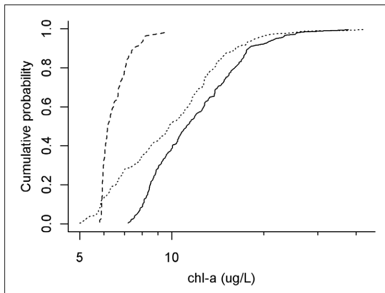
Figure 2-20. MEI predictions of chl-a distributions in different lake classes. Note that the dashed line: clear, low alkalinity lakes; solid line: clear, high alkalinity lakes; dotted line: colored lakes.
