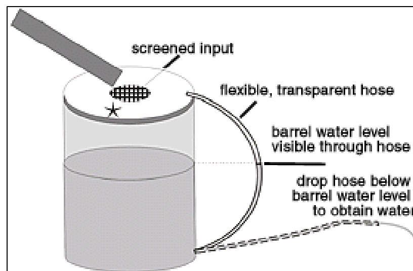
Typical rain barrel design.
