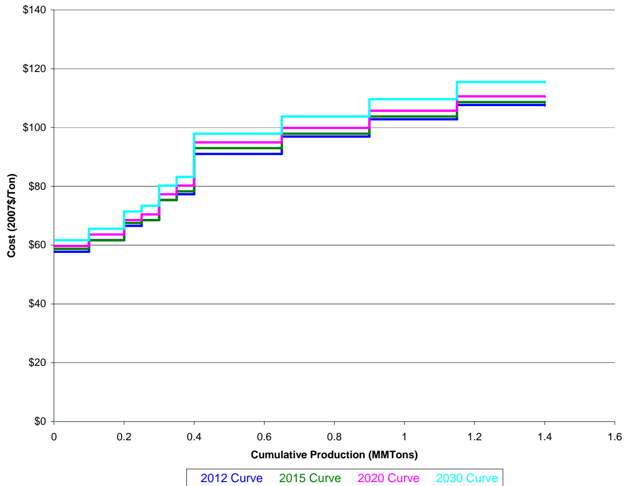
Coal Supply Curve - VA_BA
