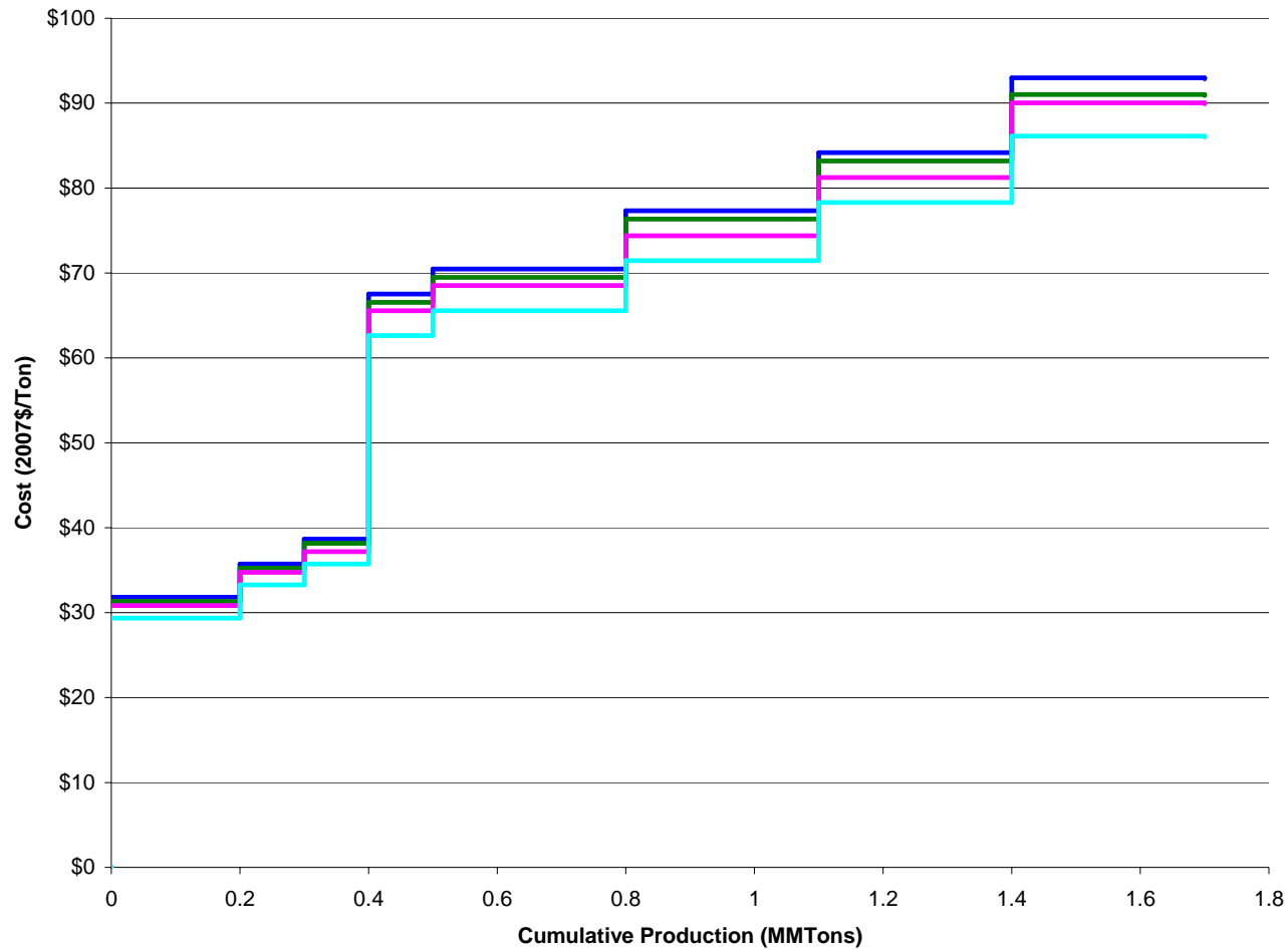
Coal Supply Curve - OH_BD
