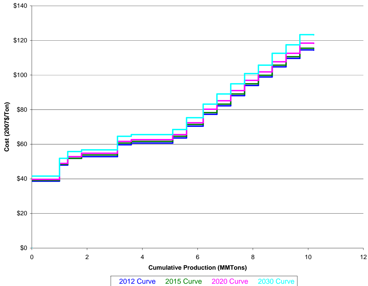
Coal Supply Curve - KE_BB
