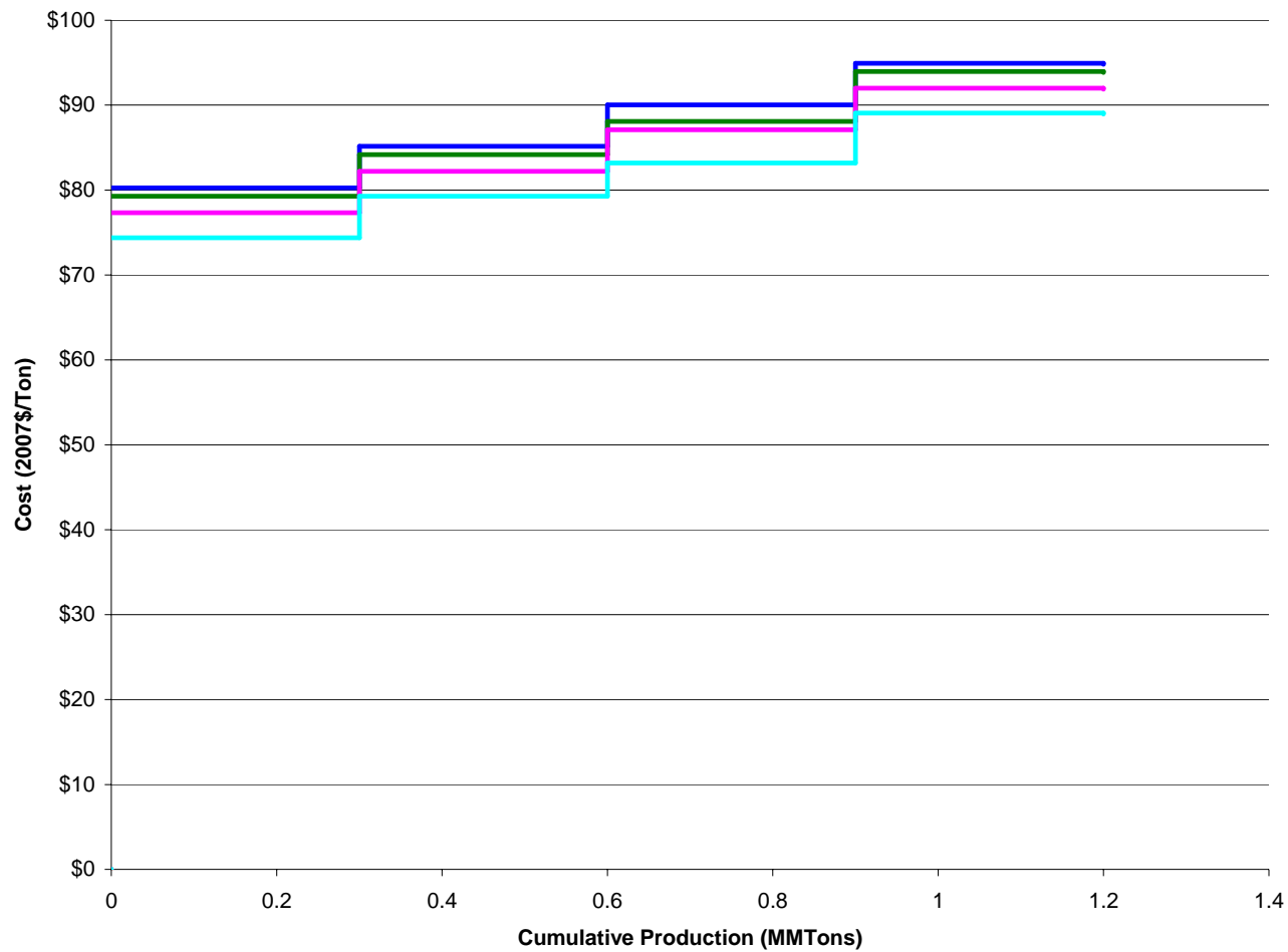
Coal Supply Curve - MD_BB
