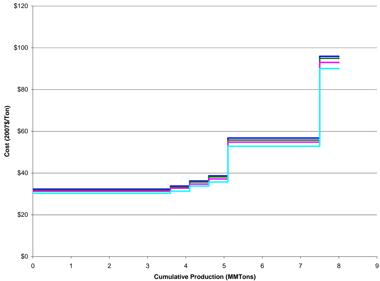
Coal Supply Curve - IN_BD
