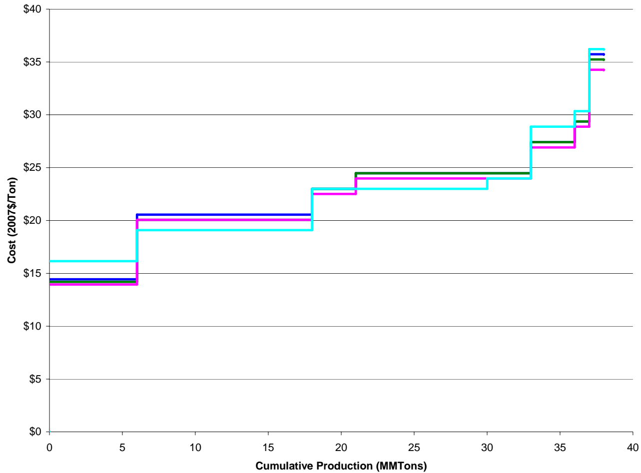
Coal Supply Curve - CG_BA
