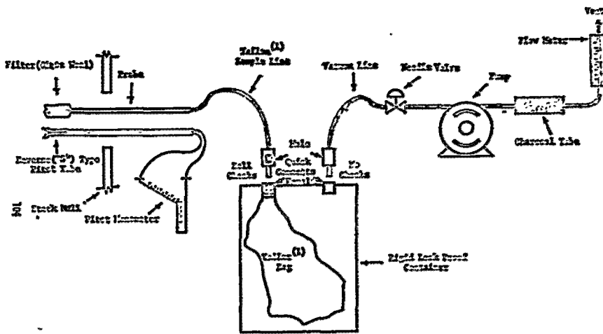
Figure 106-2. Integrated bag sampling train.
