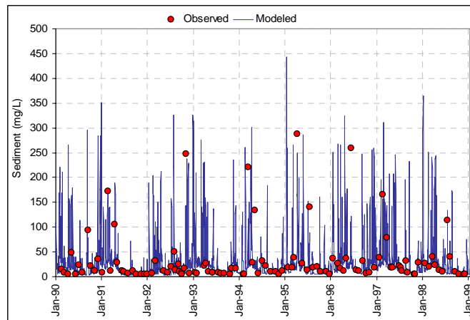
Figure 22. Observed versus simulated TSS.
