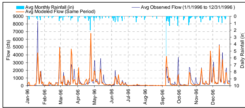
Figure 21. Observed versus simulated daily flow
